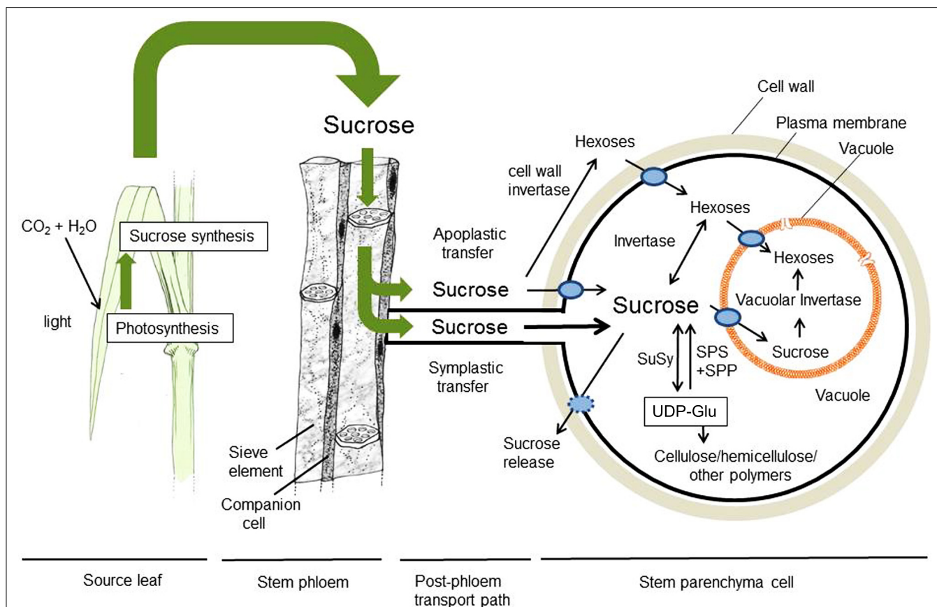
FIGURE 1 | Process diagram for sucrose movement and metabolism in sugarcane from its synthesis in source leaves to its deposition in stems. Sucrose movement is shown with green arrows, and its subsequent metabolism and compartmentalization with narrow black arrows. Transporters are shown with blue ovals, cell wall is designated with a wide tan circle, and the vacuole is shown in orange. Sucrose synthesized in photosynthetic leaves is translocated in phloem to stem parenchyma cells, where its post-phloem transfer can follow two paths: symplastic (through plasmodesmata, as thought to predominate in the mature sugarcane internodes) and/or apoplastic (through the cell wall space considered a possible contributor earlier in sugarcane stem growth). Sucrose can move unaltered to storage
