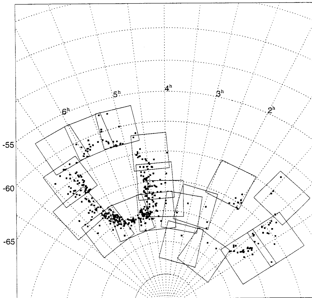
Fig. 1. Distribution of the newly identified carbon stars. Candidates were selected to have colours B_J - R > 2.4 and 14 < R < 17 and were spectroscopically confirmed as Cloud carbon stars. Toward the inner parts of both the SMC and LMC not all candidates were followed up
