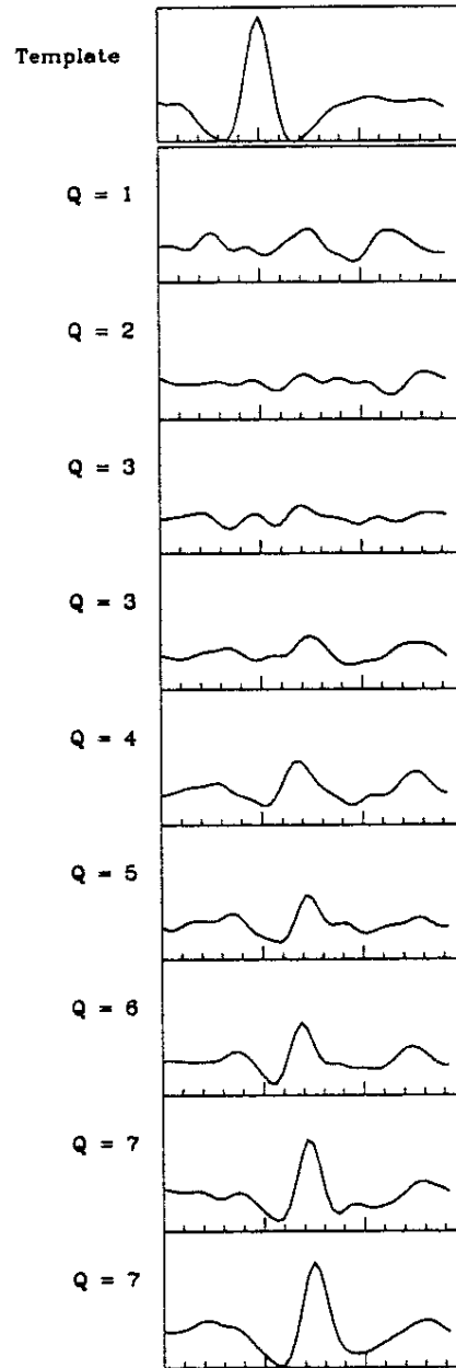
Fig. 2. Sequence of correlation functions used to assign the quality of the radial velocities. Ordinates are normalised with respect to the zero-lag peak of the template spectrum cross-correlated with itself (top panel). The small tick marks on the abscissa denote intervals of 100 \text{ km/s}
