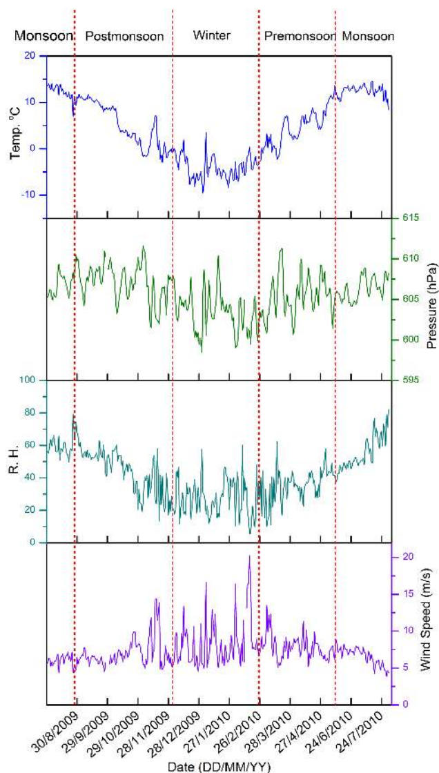
Figure 2. Time series of ambient temperature, atmospheric pressure, relative humidity and wind speed at QOMS from August 2009 to July 2010.
