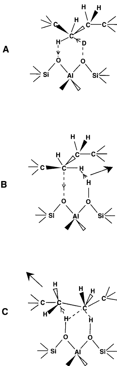
Fig. 1. Schematic representation of the proposed transition states for (A) H/D exchange, (B) butane dehydrogenation (note that the CH bond stretches and H 2 and a \sigma -bonded carbenium ion are generated) and (C) cracking (note that the carbon-carbon bond stretches, ethane and a \sigma -bonded carbenium ion are generated). The arrows indicate the atomic motion.
