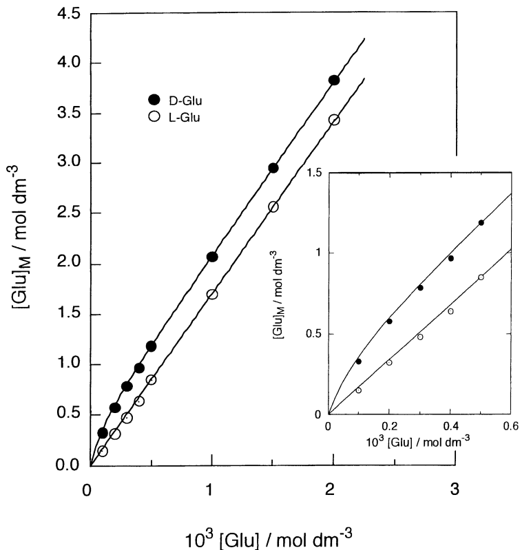
Figure 3 Adsorption isotherms of D-Glu and L-Glu in the Z-L-Glu imprinted polymeric membrane. ((Z-L-Glu) / (PSf) = 0.5; k_D = 1.8 \times 10^3 ; [PSf] = 7.4 \text{ mol dm}^{-3} ; n = 5.7 \times 10^{-2} ; K_C = 7.9 \times 10^3 \text{ mol}^{-1} \text{ dm}^3 .)
