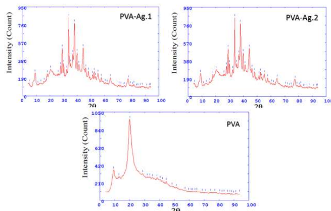
Fig. 4: XRD pattern of PVA and AgNps;
