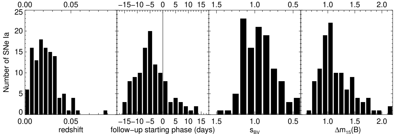
Figure 3. Characteristics of the SNeIa in the NIR spectroscopy program. The distributions in redshift, light curve follow up starting phase, s_{BV} , and \Delta m_{15}(B) are shown in panels from left to right.
