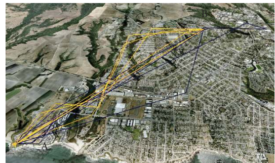
FIGURE 18: GPS data from the test deployment. The yellow track was logged by the GPS on a CSN carried by a researcher. The black track is the GPS data from the CSN carried by a domestic dog. An SRN was located at Long Marine Lab, Santa Cruz, CA, USA (A). The dog lived at B and his owner worked at A. Data was successfully transferred to the SRN via hops 1 and 2.
