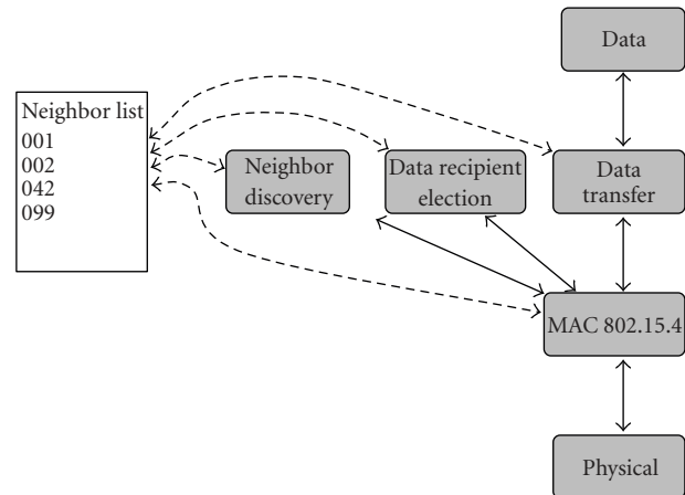
FIGURE 6: Network stack and associated data structure. The CARNIVORE stack uses a neighbor table to mediate the use of the wireless channel. The list is populated during neighbor discovery and updated by various layers. Received frames are processed in the MAC layer which then updates the neighbor list.
