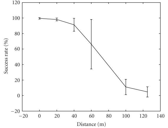
FIGURE 10: CSN-to-CSN range test. This test was conducted across a field with waist-high vegetation. Both collars were elevated 2 m. Bars indicate one standard deviation.
