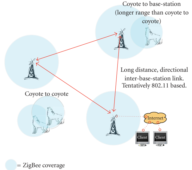
FIGURE 1: Overview of the CARNIVORE network. A predator, such as a coyote, wears a collar containing a CSN while fixed base stations or SRNs act as data sinks. CSN-to-SRN wireless range is greater than coyote-to-coyote wireless range because the base stations employ high-gain collinear antennas. An SRN has been developed for capturing data from CSNs; however, the final SRN has yet to be implemented to deliver data via the internet.
