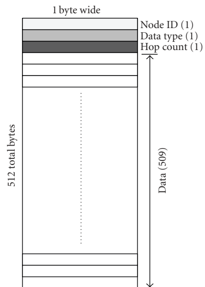
FIGURE 5: Collar data segment. These segments are stored in the FIFO buffers of the microSD card. Numbers in parentheses are bytes.
