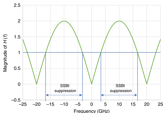
Fig. 7 Magnitude of transfer function H(f) for CADD. SSBI suppression is defined as |H(f)| > 1
