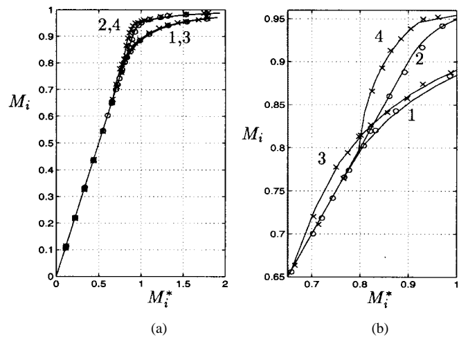
Fig. 16. Experimental and theoretical M_i = f(M_i^*) characteristics of SPWM and SVPWM. (a) Full modulation range. (b) Magnified view of the nonlinear modulation region. 1: SPWM, 2: SVPWM, 3: SPWM with MPW, and 4: SVPWM with MPW. The experimental data is shown with "o" and "x" symbols, while the continuous curves correspond to the theoretical formulas.
