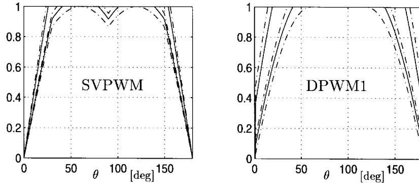
Fig. 11. Overmodulation region modulation wave profiles of SVPWM and DPWM1 for five different M_i^* values.
