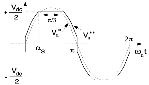
Fig. 7. DPWM1 method overmodulation waveforms.
