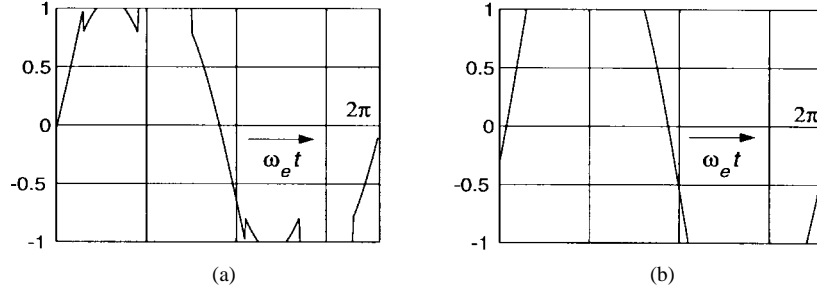
Fig. 8. DPWM2 method overmodulation waveforms. (a) Region I. (b) Region II.
