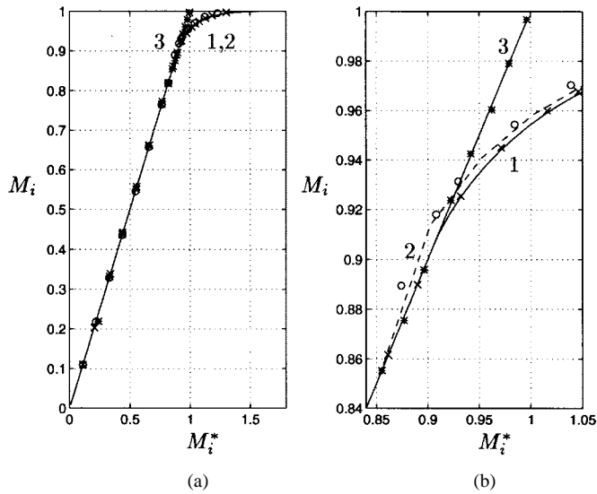
Fig. 18. (a) Experimental and theoretical M_i = f(M_i^*) characteristics of DPWM1 with and without linearization and (b) the magnified view of the overmodulation region. 1: The theoretical M_i = f(M_i^*) curve. 2: The theoretical M_i = f(M_i^*) curve with MPW. 3: Ideal linear modulator line. The experimental results are shown with "o," "x," and "*" symbols.
