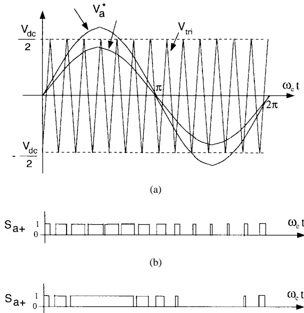
Fig. 2. SPWM modulation waveforms and switching device gate logic signals. (a) Linear modulation range. (b) Overmodulation range.
