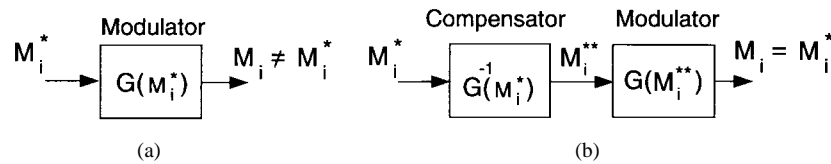
Fig. 14. Overmodulation range voltage-gain block diagrams. (a) Modulator nonlinear gain characteristic. (b) The compensator cancels the nonlinearity by inverse gain multiplication.
