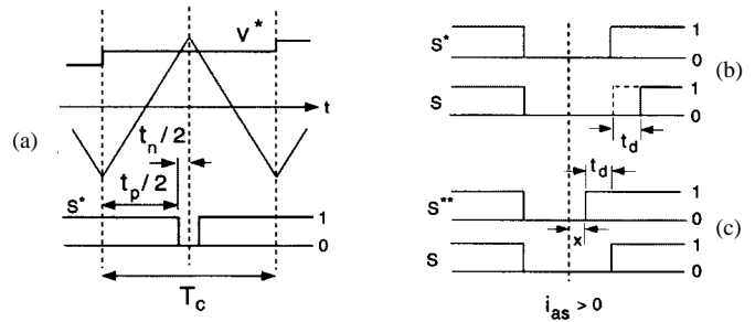
Fig. 12. Regular sampling PWM reference and gate signals. (a) The reference gate signal at high-modulation level. (b) No compensation results in asymmetric gate signal (for i_{as} > 0 ). (c) Signal after exact compensation.
