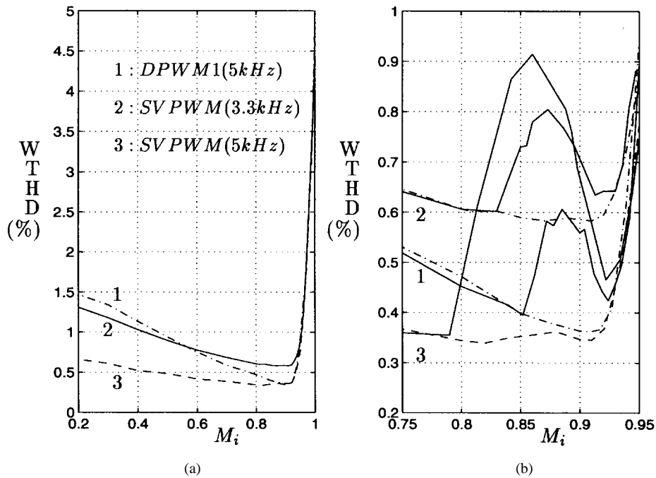
Fig. 15. WTHD characteristics of SVPWM and DPWM1. (a) Ideal inverter model case. (b) Magnified view with MPW (—) and without MPW (---) control algorithm.
