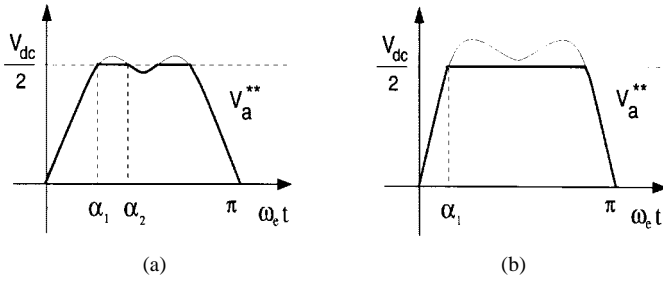
Fig. 6. THIPWM waveforms in the overmodulation region. (a) Region I. (b) Region II.
