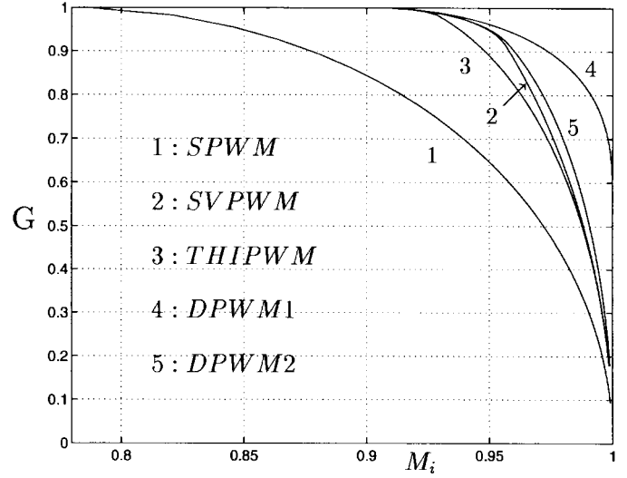
Fig. 9. The overmodulation region voltage-gain characteristics of the popular modulators.
