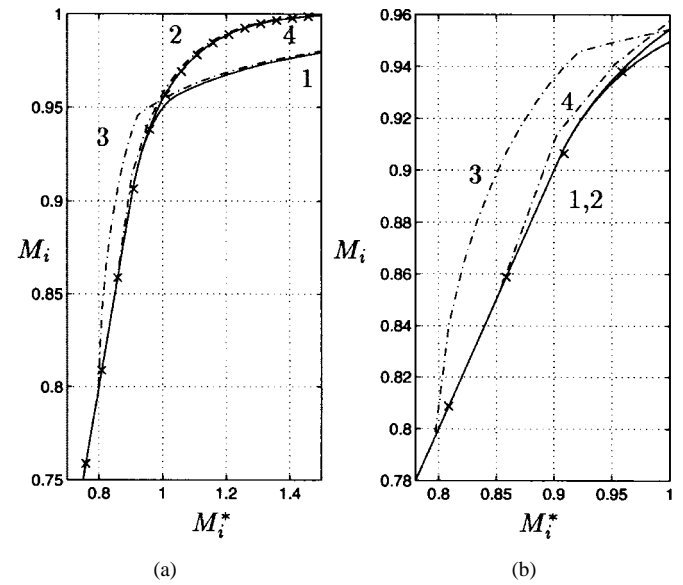
Fig. 13. (a) SVPWM and DPWM1 theoretical M_i = f(M_i^*) characteristics and (b) the magnified view in the low end of the overmodulation region. 1: SVPWM, 2: DPWM1, 3: SVPWM with MPW, and 4: DPWM1 with MPW. The blanking-time-dependent nonlinearity of DPWM1 is shown with the "x" symbol.
