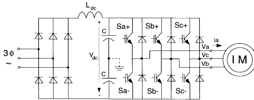
Fig. 1. Main power converter structure of the widely utilized diode-rectifier front-end-type PWM-VSI drive.
