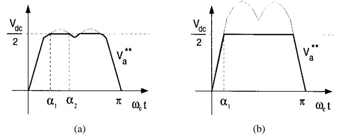
Fig. 5. SVPWM triangle-intersection method modulation waveforms in the overmodulation region. (a) Region I. (b) Region II.
