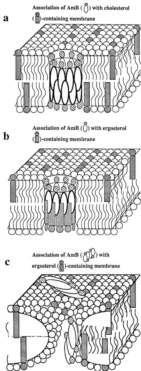
FIG. 5. Models illustrating the possibilities for the formation of channels by AmB interacting with sterol-containing membranes. (a) Model A, cholesterol-containing membrane; (b) model B, ergosterol-containing membrane; (c) AmB aggregates inserting into ergosterol- or cholesterol-containing membrane. The head-to-tail assembly of the AmB molecules in membranes and the complexation of ergosterol to AmB in a single leaflet have not yet been demonstrated experimentally.
