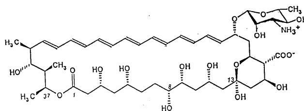
FIG. 1. Structure of AmB.
