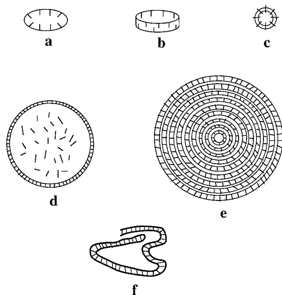
FIG. 3. Schematic representation of different lipid formulations of AmB. (a) Fungizone (deoxycholate-AmB mixed micelles); (b) ABCD or Amphocil (cholesteryl sulfate-AmB mixed micelles); (c) AmBisome (AmB-containing SUV); (d) AmB-containing LUV; (e) L-AmpB (AmB-containing multilamellar vesicles); (f) ABLC, ribbon-like formations (DMPC-DMPG-AmB, 4.6:2.3:3). Symbols: —, AmB molecule; O, membranes of various lipid compositions.
