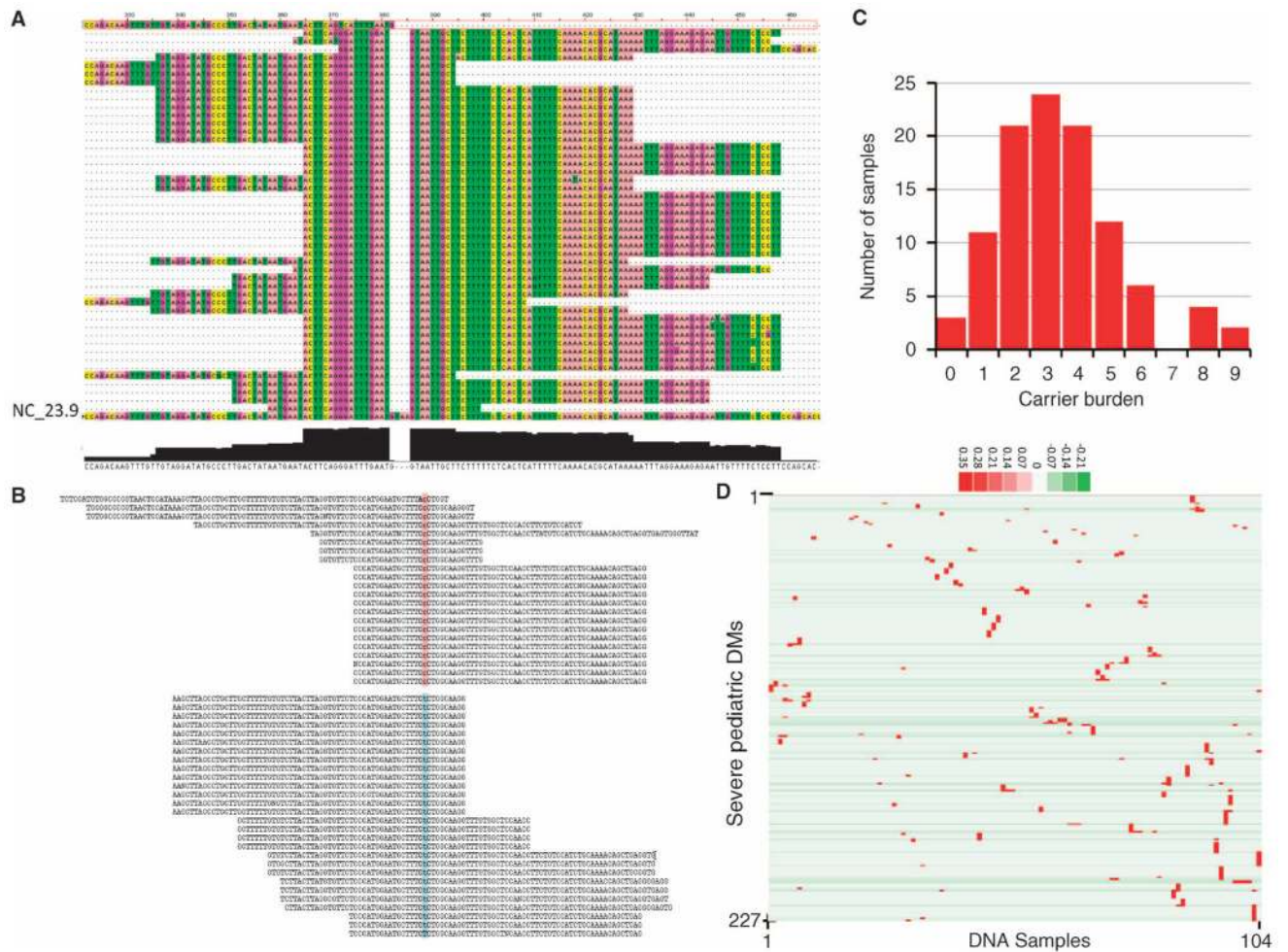
Fig. 7. Disease mutations and estimated carrier burden in 104 DNA samples. (A) Sample NA0792, from an affected male with X-linked recessive Lesch-Nyhan syndrome (OMIM #300322), had been characterized as a deletion of HPRT1 exon 8 by cDNA sequencing (19), but has an explanatory splicing mutation (intron 8, IVS8+1_4delGTAA, chrX: 133460381_133460384delGTAA). (B) Sample NA09545, from an affected male with X-linked recessive Pelizaeus-Merzbacher disease (PMD; OMIM #312080), characterized as a substitution disease mutation [PLP1 exon 5, c.767C>T, P215S (20)], also featured PLP1 gene duplication [which is reported in 62% of sporadic PMD (21)]. (C) Distribution of carrier burden of severe pediatric diseases among 104 DNA samples. (D) Ward hierarchical clustering of 227 severe pediatric disease mutations in 104 DNA samples.
