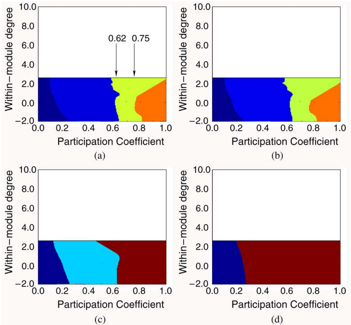
Figure 8. Basins of attraction for density landscapes obtained for non-hub nodes obtained with (a) \sigma_P = 0.03 , (b) \sigma_P = 0.035 , (c) \sigma_P = 0.05 , and (d) \sigma_P = 0.08 . Note how the values of P identified in our simple analysis provide a good match to the boundaries of the basins of attraction in the node density landscapes.
