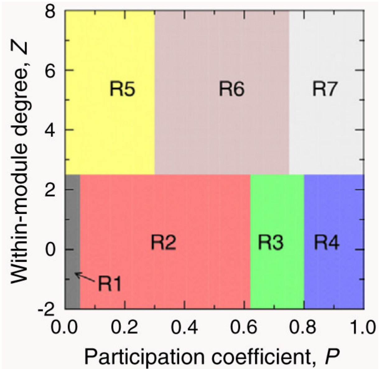
Figure 5. Role-specific regions in the zP parameter space.
