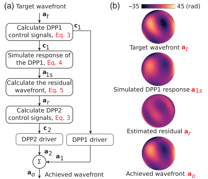
Fig. 3 Open-loop control method for simultaneous control of cascaded DPPs. (a) Control flowchart and (b) visualization of different steps of replicating a target wavefront.
