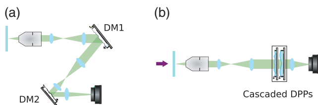
Fig. 1 (a) The conventional usage of two reflective elements for AO versus (b) the cascaded configuration of two refractive DPPs. DM: deformable mirror.
