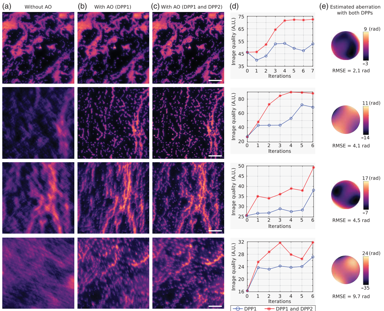
Fig. 7 Imaging fluorescent micro-beads ( \varnothing = 1 \mu\text{m} ) behind an aberrating phase plate that mimics specimen-induced aberrations while deep tissue imaging. (a) Aberrated frames, corrected frames using (b) a single DPP and (c) the cascaded configuration, (d) quality score of the obtained frames after each iteration of the aberration estimation algorithm, and (e) the estimated wavefront error by executing the sensorless aberration estimation algorithm using stacked DPPs. Length of the scale bars is 20 \mu\text{m} .
