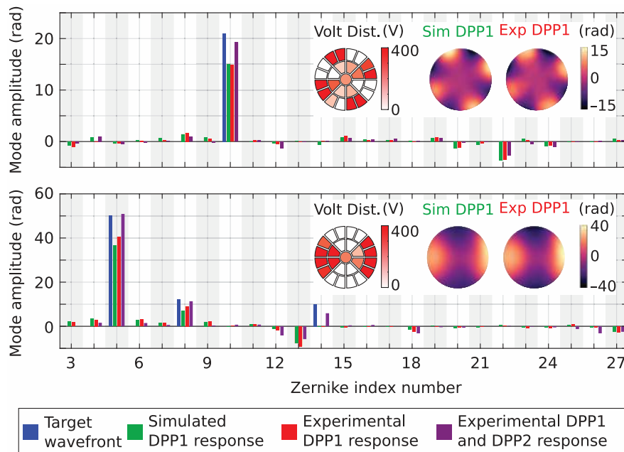
Fig. 4 Experimental evaluation of the introduced open-loop control for replicating two example wavefronts using DPP1 and DPP2. A target wavefront is chosen and the control signals of the DPP1 are calculated. The keystone patterns on each plot show the voltage distribution of the DPP1. These control signals are used to estimate the DPP1 response by its response model. The two wavefront profiles on each plot compare the estimated response from experimental measurements. Bar plots compare the Zernike decomposition of the target and reproduced wavefronts at each step of the control algorithm depicted in Fig. 3(a). Interferometric measurements are performed using a HeNe laser ( \lambda = 632 \text{ nm} ).
