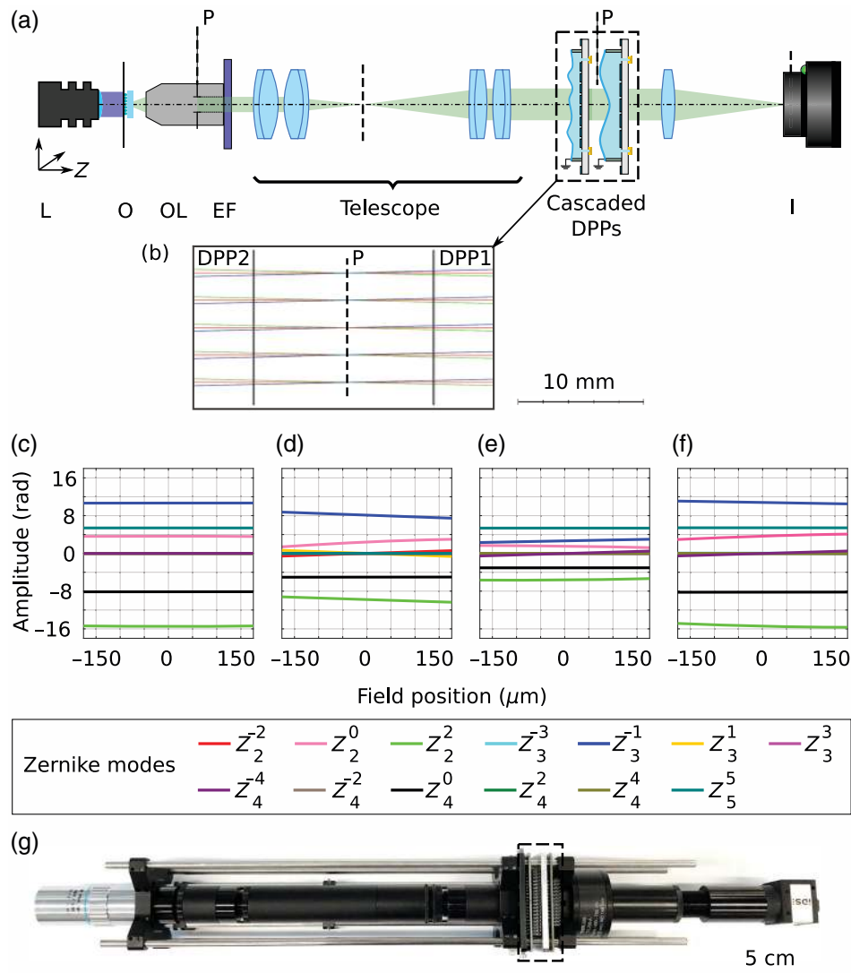
Fig. 6 (a) Schematic layout of the developed AO microscope. P, pupil plane; O, object; OL, objective lens; EF, emission filter; and I, image. (b) Detailed view of the ray-tracing simulation model at the location of cascaded DPPs each having a 7-mm offset from the conjugated pupil plane. Simulation results depicting the amplitudes of the Zernike modes with respect to field positions for (c) the ideal case of having both DPPs directly at the pupil plane, (d) only DPP1 actuated while being positioned 7 mm behind the pupil plane, (e) only DPP2 actuated while being positioned 7 mm in front of the pupil plane, and (f) DPP1 and DPP2 actuated simultaneously at their offset-position. (g) Overview of the fully refractive AO microscope with the integrated cascaded DPPs.
