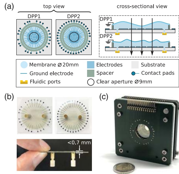
Fig. 2 (a) Schematics of the employed DPPs and their proposed cascaded configuration. DPP1 has 25 keystone-patterned electrodes that are distributed within an area of 12 mm in diameter, and DPP2 has 37 hexagonally patterned electrodes that can be circumscribed inside a circle of 12 mm in diameter. (b) Top and side views of the fabricated DPPs. (c) Stacked DPPs in their 60-mm cage system compatible packaging and electrical interfacing.
