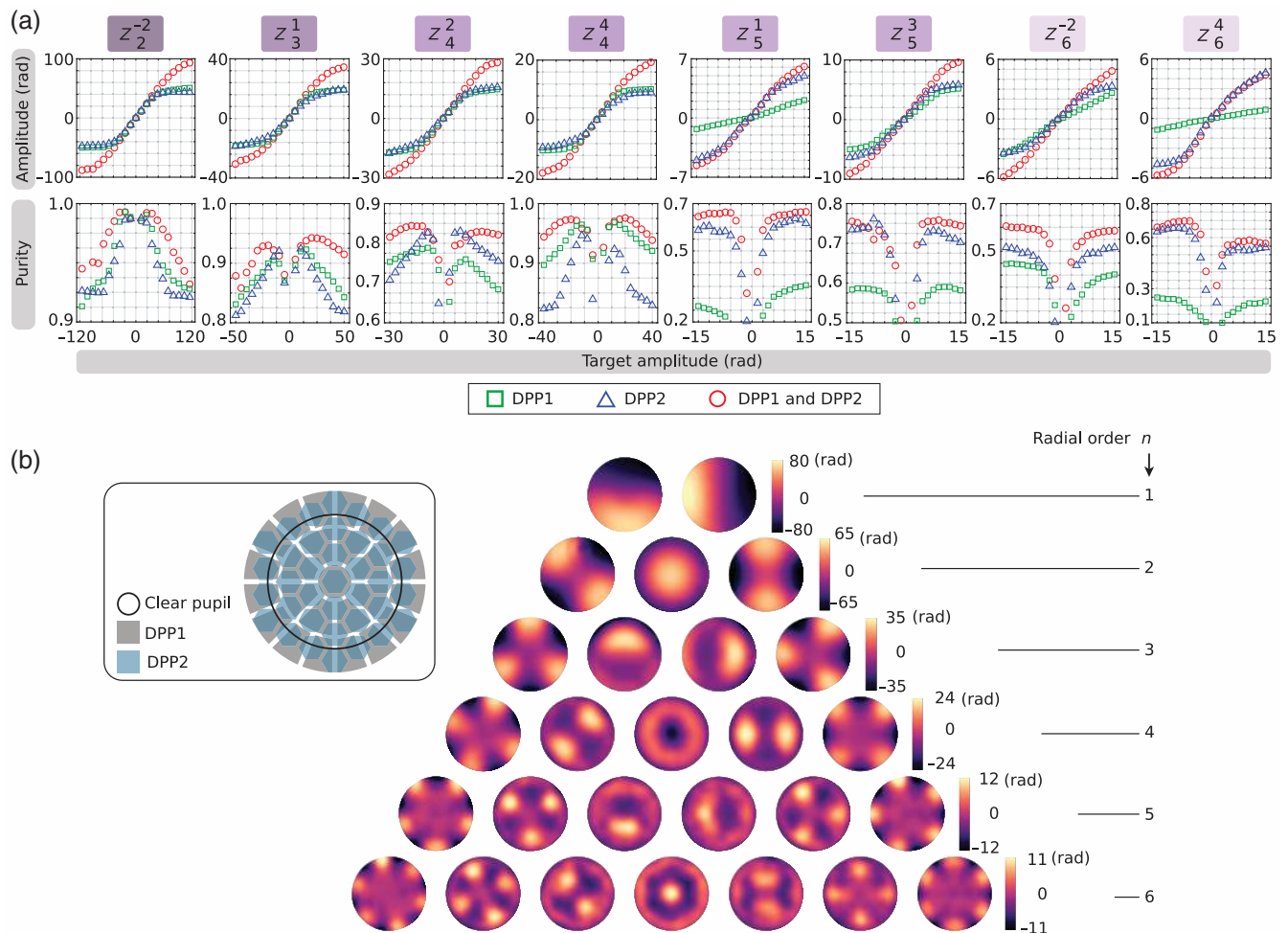
Fig. 5 Experimental results for replicating up to the sixth radial order of Zernike modes. (a) Comparing the maximum achievable mode amplitude and their corresponding purity [see Eq. (6)] using DPP1 and DPP2 individually (depicted by green squares and blue triangles, respectively), and simultaneously with the cascaded configuration and the proposed control method (red circles). (b) Overview of the wavefront profiles of the replicated Zernike modes using the cascaded DPPs. The top-left figure shows the overlay of DPP1 and DPP2 electrode patterns. Interferometric measurements are performed using a HeNe laser ( \lambda = 632 nm).
