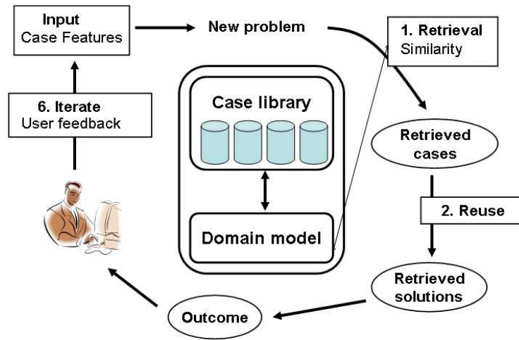
Fig. 10. Comparison-Based Retrieval
