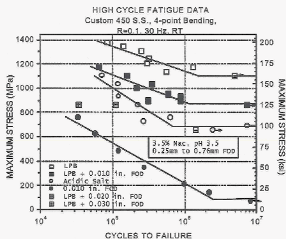
Figure 12 - Corrosion fatigue performance of Custom 450 stainless steel with FOD in acidic salt solution and FOD from 0.25mm (0.010 in.) to 0.76mm (0.030 in.).
