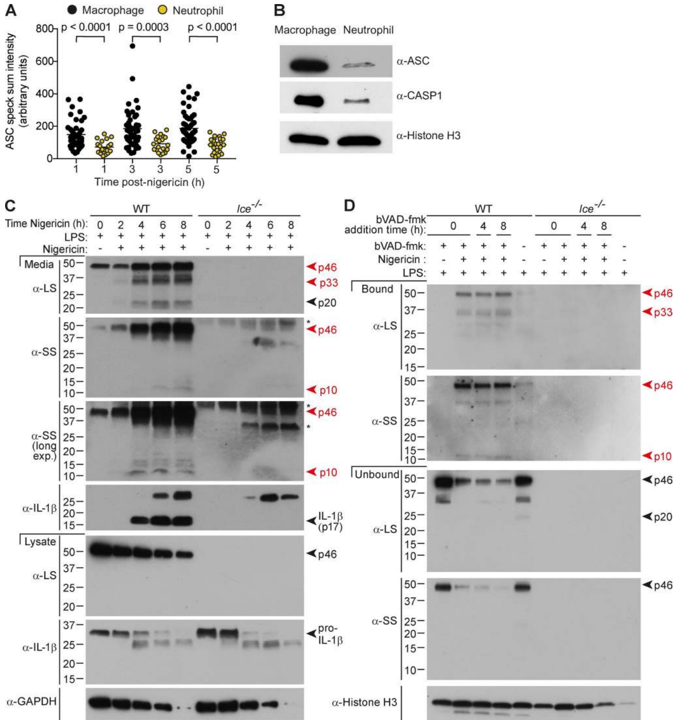
Figure 5. Cell type specifies caspase-1 activity duration. (A–D) LPS-primed (A and B) macrophages or (A–D) neutrophils were left untreated or stimulated with nigericin. (A) ASC speck intensity of lce -/- macrophages and neutrophils (4 h LPS + nigericin), quantified from microscopy images. Each circle is one speck ( n = 20 –55), and significance between samples was assessed by nonparametric, unpaired Mann–Whitney test. (B) Immunoblot for inflammasome component expression in whole-cell extracts (4 h LPS). (C) Cell lysates and cell-free supernatants were harvested at various times after nigericin stimulation (0, 2, 4, 8 h), and analyzed by Western blot. *, Nonspecific band. (D) bVAD-fmk was applied at the indicated time points. Supernatant was removed, and cells were lysed 8 h after nigericin stimulation, and active caspase-1 was pulled down using streptavidin beads. Streptavidin-bound and -unbound fractions from mixed supernatants/extracts were analyzed by Western blot. All data are representative of at least three (A, B, C [WT], D [WT]) or two (C [ lce -/- ], D [ lce -/- ]) independent experiments.
