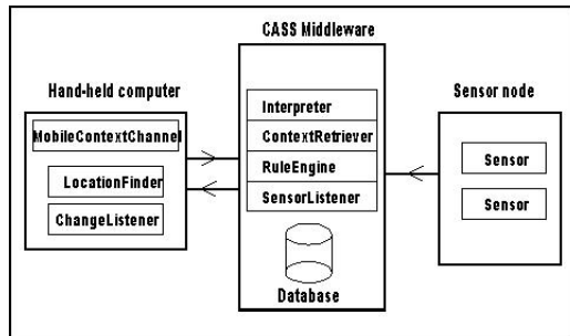
Fig. 1. CASS architecture
