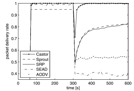
Fig. 5. Wormhole attack resilience. Failure recovery time.
