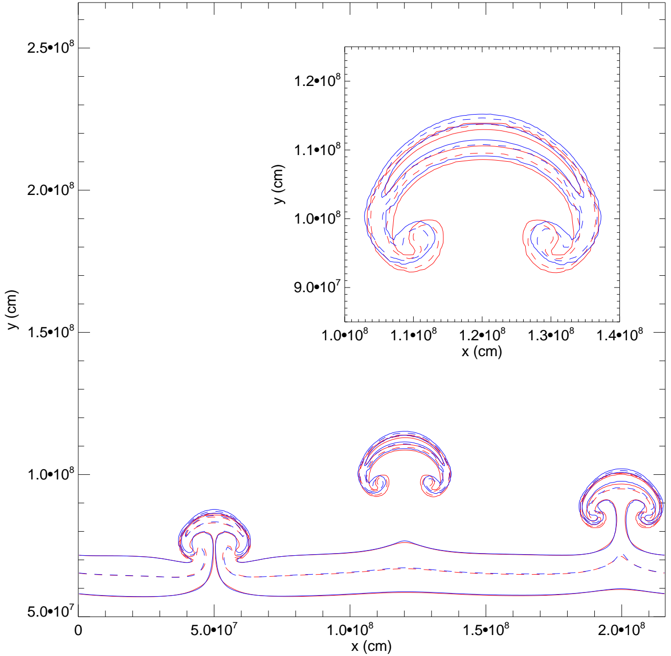
Fig. 14.— Comparison of FLASH (red) and CASTRO (blue) ^{24}\text{Mg} mass fraction contours for the reacting bubble test. Contours are drawn at values of X of 5 \times 10^{-9} , 5 \times 10^{-8} , 5 \times 10^{-7} , 5 \times 10^{-6} , with alternating solid and dashed lines. The inset shows the detail of the middle bubble. As with the temperature, we see good agreement between FLASH and CASTRO.
