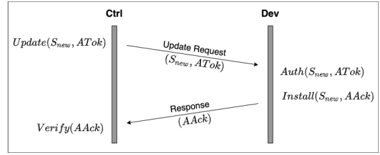
Figure 2: CASU Secure Update Protocol.
