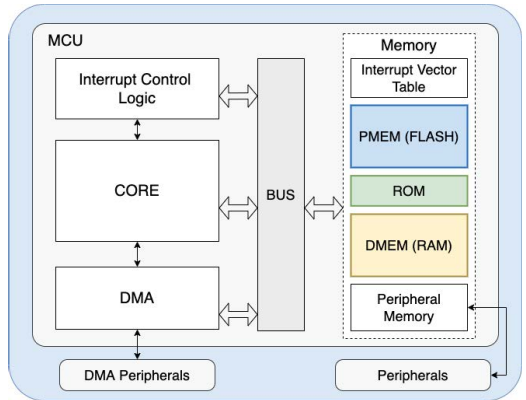
Figure 1: System architecture of a typical low-end MCU.
