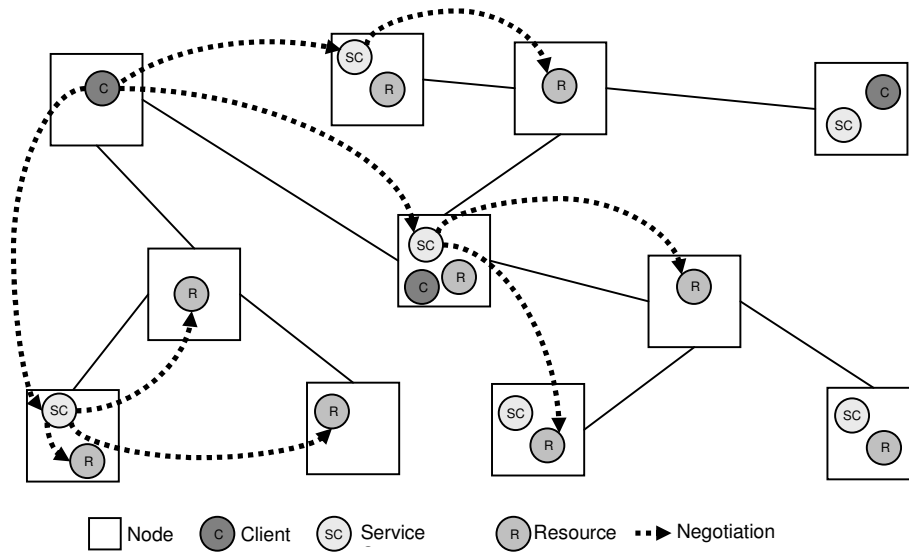
Figure 3: Catalactic middleware as a network of agents
