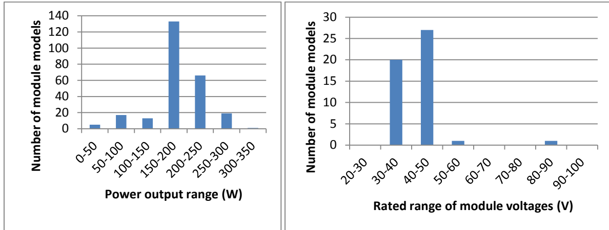
(a) (b) Figure 15. Rated power output (a) and voltages (b) of PV modules satisfying the Guidelines for California’s Solar Electric Incentive Programs. Data source: [40].
