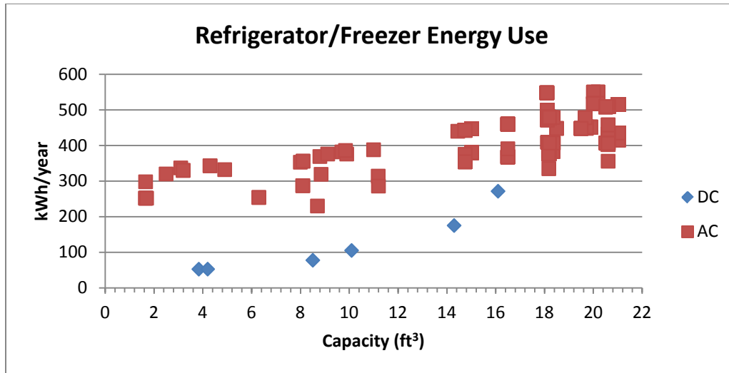
Figure 12. Energy use for DC and AC Refrigerator/Freezers.
