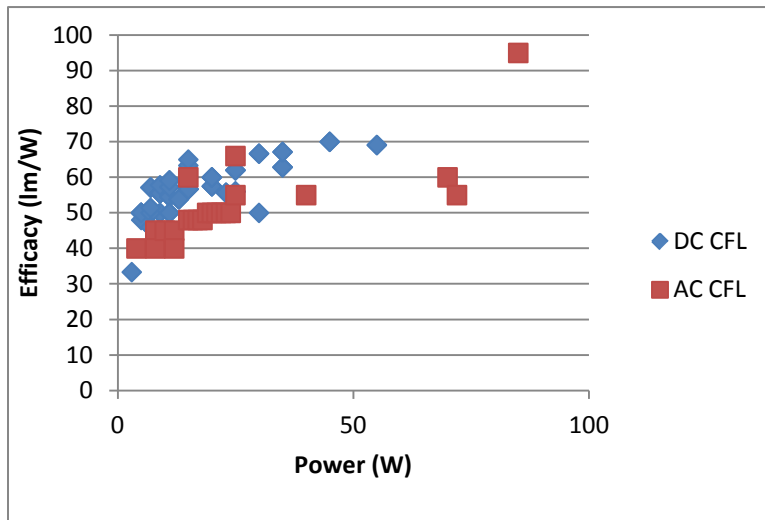
Figure 7. Efficacy comparison for DC and AC CFLs.
