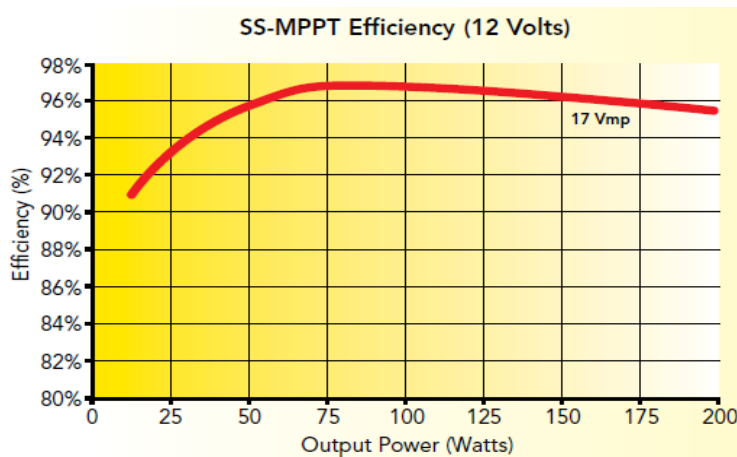
Figure 23. Efficiency curve of the MorningStar SunSaver charge controller with MPPT.
