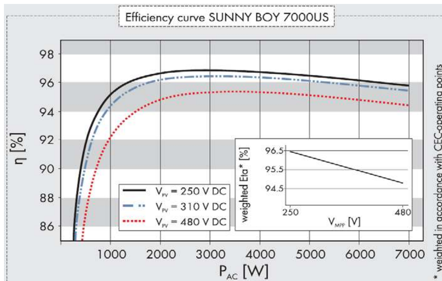
Figure 21. Efficiency curve for the SMA Sunny Boy 7000US string inverter (with MPPT).
