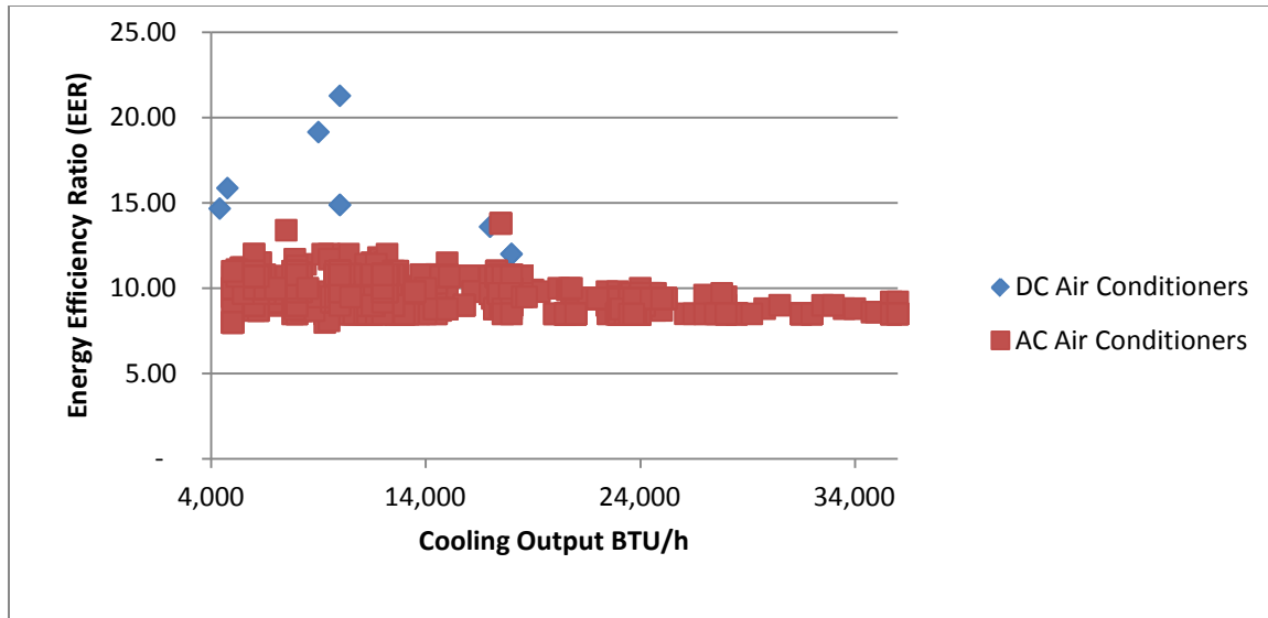
Figure 6. Energy efficiency comparison for DC and AC air conditioners.
