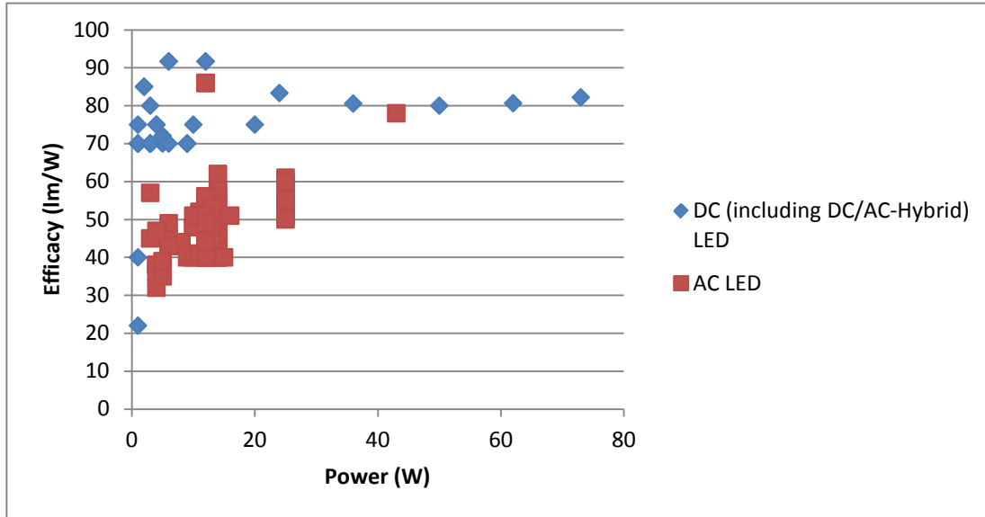
Figure 8. Efficacy comparison for DC and AC LEDs.
