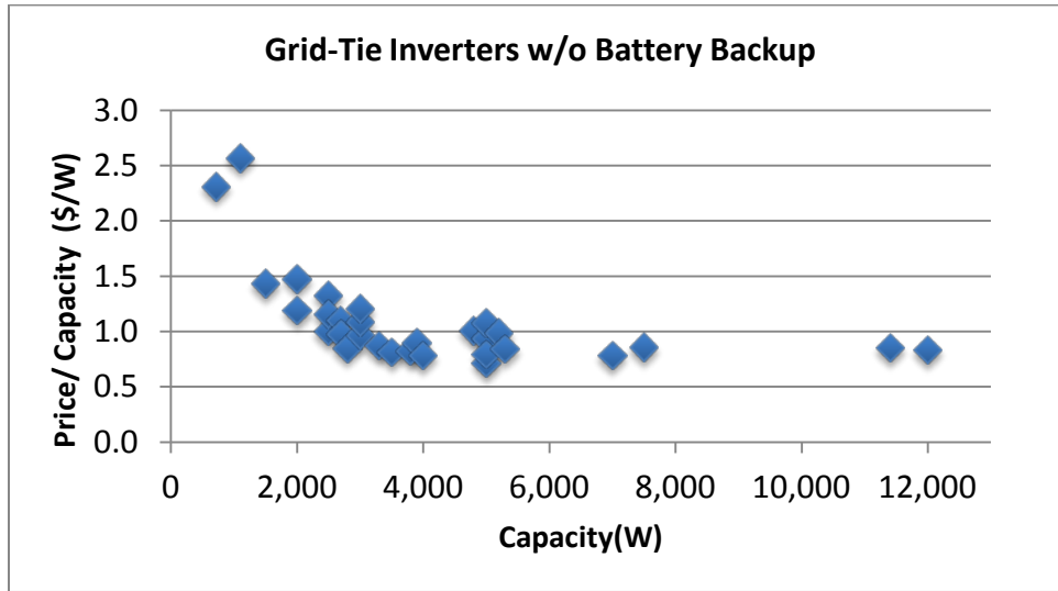
Figure 20. Retail price curve for grid-tie inverters without battery backup (2010 data).
