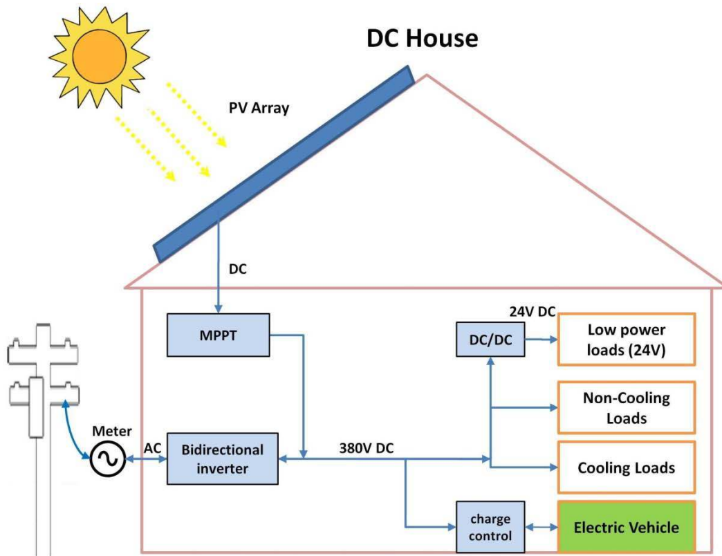
Figure 3. Direct-DC Power System.
