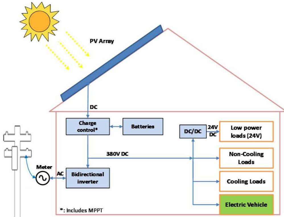
Figure 5. DC Power System with Storage.
