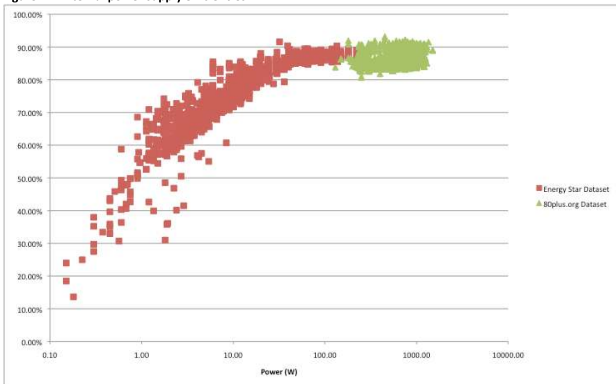
Figure 14. External power supply efficiencies.
