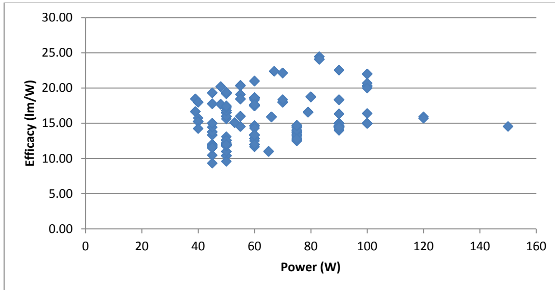
Figure 11. Efficacy of AC incandescent reflector lamps. Data source: The California Energy Commission Appliance Efficiency Database [12].
