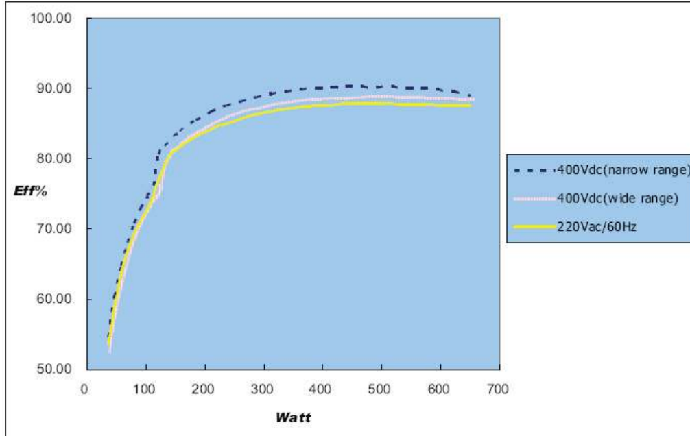
Figure 22. DC data center power supply efficiency curve.
