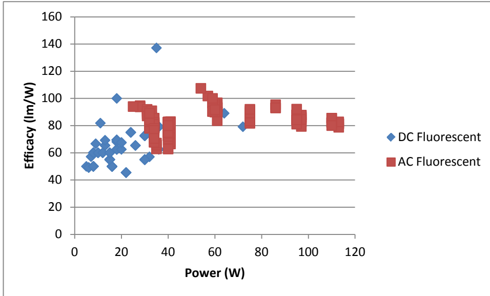
Figure 9. Efficacy of DC and AC fluorescent lighting products.
