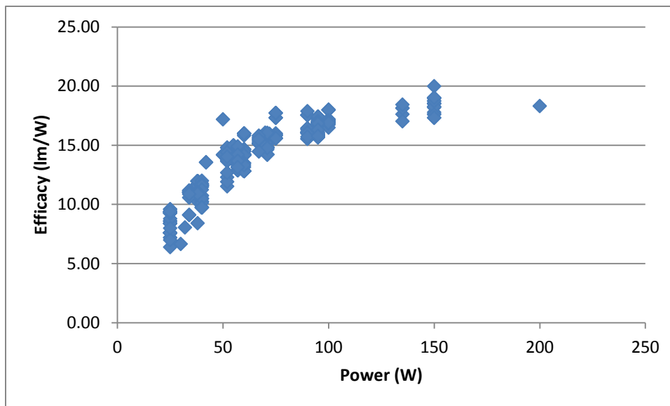
Figure 10. Efficacy of AC incandescent lamps.
