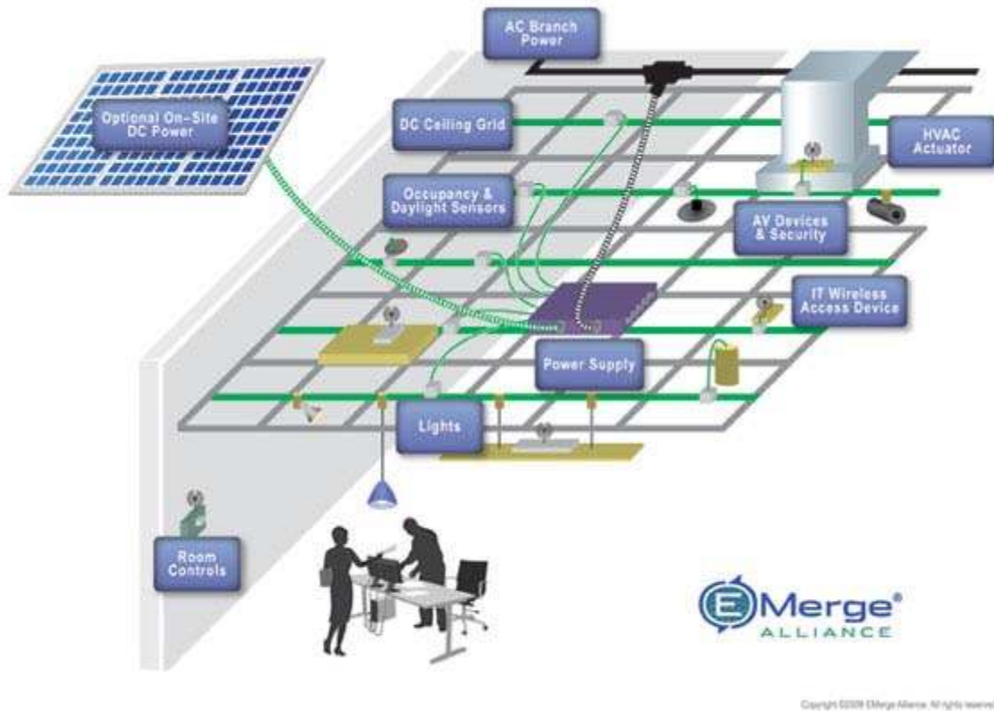
Figure 26. A typical ceiling-based EMerge system schematic Source: [65].
