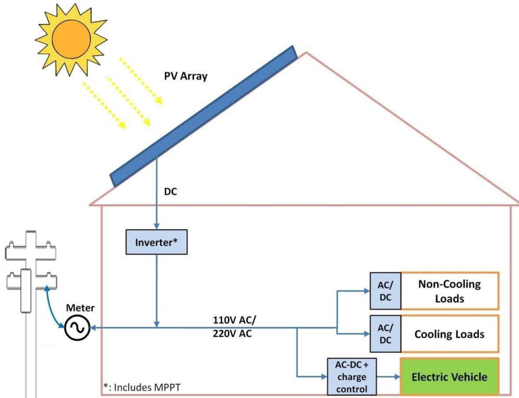
Figure 2. Typical AC Power System.
