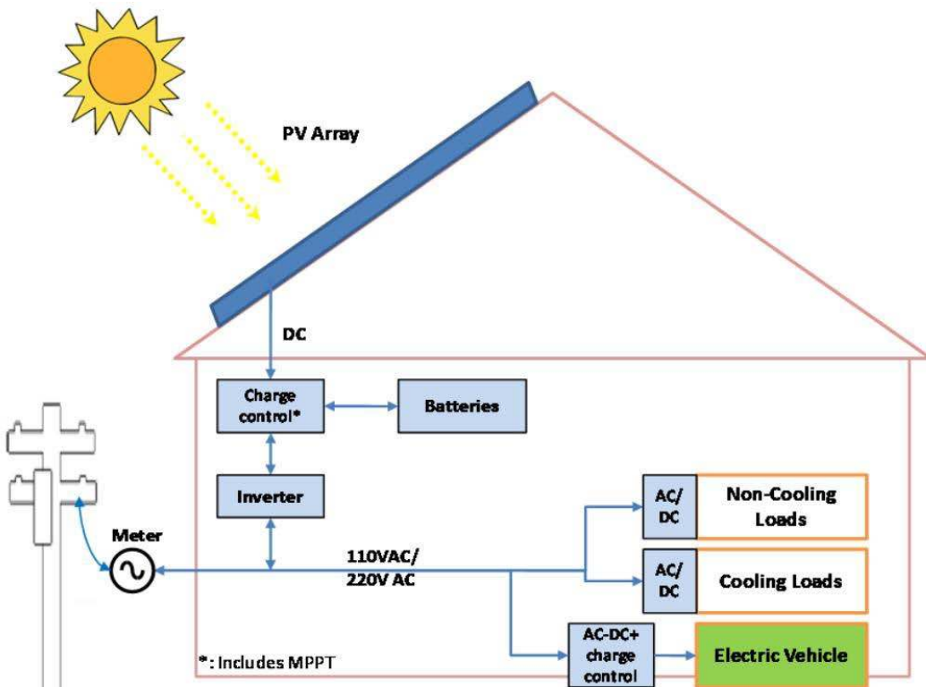
Figure 4. AC Power System with Storage.
