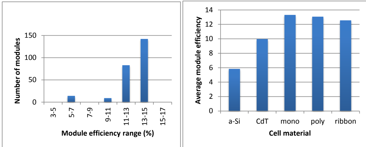
(a) (b) Figure 16. Efficiencies of PV modules satisfying the Guidelines for California’s Solar Electric Incentive Programs . (a) Histogram of modules by efficiency, (b) Efficiency by cell type (amorphous silicon (a-Si, n=11), cadmium telluride (CdT, n=6), monocrystalline (mono, n=87), polycrystalline (poly, n=127), and ribbon (n=17). Source: [38]
