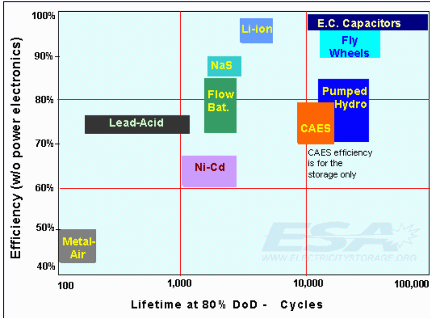
Figure 25. Storage technologies comparison.
