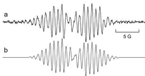
Figure 4. EPR spectra from photolysis of acid 4d in PhH at 300 K. a) Experimental spectrum from 4d . b) Computer simulation.
