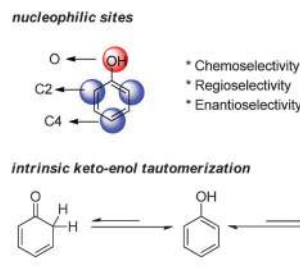
Fig. 3 Nucleophilic sites on the phenol ring and the intrinsic keto-enol tautomerization of phenol.
