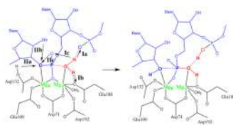
Figure 2. Schematic representation of the active site coordination. Arrows in the reactant state representation indicate possible PT pathways in processes I and II.
