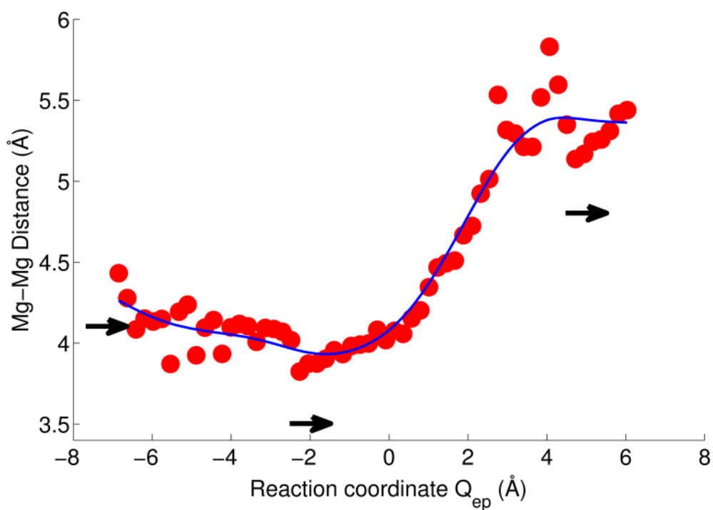
Figure 6. Mg^{2+} - Mg^{2+} distance along the reaction coordinate Q_{ep}=ET+(PT1a+PT1b)/2+PT2 for the catalytic reaction of the protonated Asp132 system. Arrows indicate the Mg^{2+} - Mg^{2+} distances in reactant, transition-state like, and product structures 10,12 (PDB codes 1ZBL, 2G8H and 2G8F, and 2G8V, respectively; left to right). The data points are calculated from reweighted string simulations and the curve is a spline fit to guide the eye.
