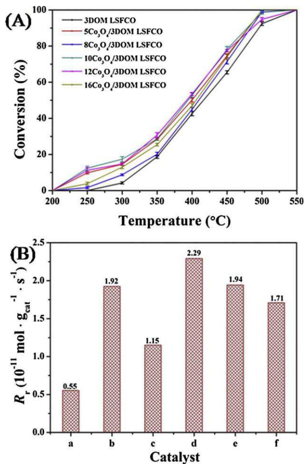
Fig. 7. (A) Light-off curves of 1,2-DCE oxidation and (B) reaction rate ( R_r ) at 300 °C over (a) 3DOM LSF CO , (b) 5Co 3 O 4 /3DOM LSF CO , (c) 8Co 3 O 4 /3DOM LSF CO , (d) 10Co 3 O 4 /3DOM LSF CO , (e) 12Co 3 O 4 /3DOM LSF CO , and (f) 16Co 3 O 4 /3DOM LSF CO .
