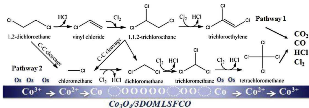
Scheme 2. Proposed mechanism for 1,2-DCE oxidation over \text{Co}_3\text{O}_4/3\text{DOM LSFCE} catalyst.
