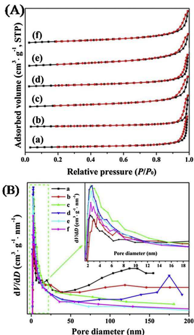
Fig. 4. Nitrogen adsorption-desorption isotherms (A) and Pore size distribution (B) of (a) 3DOM LSFCO, (b) 5Co 3 O 4 /3DOM LSFCO, (c) 8Co 3 O 4 /3DOM LSFCO, (d) 10Co 3 O 4 /3DOM LSFCO, (e) 12Co 3 O 4 /3DOM LSFCO, and (f) 16Co 3 O 4 /3DOM LSFCO.
