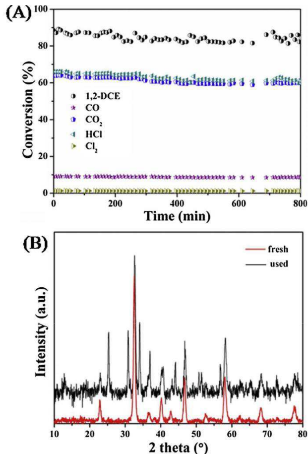
Fig. 10. (A) Stability of 10Co 3 O 4 /3DOM LSFSCO for 1,2-DCE oxidation at 480 °C; (B) XRD patterns of the fresh and used 10Co 3 O 4 /3DOM LSFSCO.
