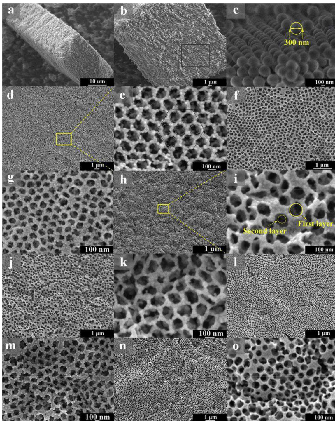
Fig. 2. Typical FE-SEM images of (a–c) PMMA microsphere, (d and e) 3DOM LSFCO, (f and g) 5Co 3 O 4 /3DOM LSFCO, (h and i) 8Co 3 O 4 /3DOM LSFCO, (j and k) 10Co 3 O 4 /3DOM LSFCO, (l and m) 12Co 3 O 4 /3DOM LSFCO, and (n and o) 16Co 3 O 4 /3DOM LSFCO.
