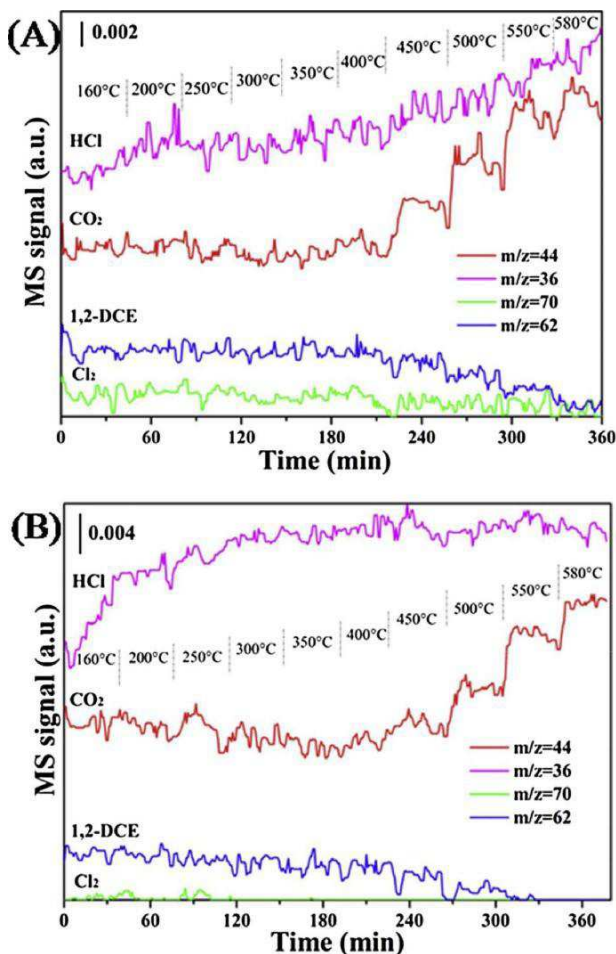
Fig. 9. On-line MS results of typical oxidation products in temperature range of 160–580 °C over (A) 3DOM LSFSCO and (B) 10Co 3 O 4 /3DOM LSFSCO.
