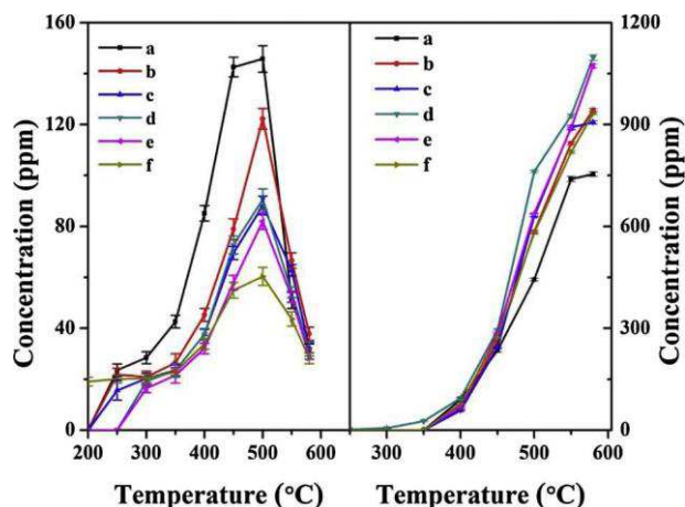
Fig. 8. CO and CO 2 distribution over the synthesized catalysts: (a) 3DOM LSFCE, (b) 5Co 3 O 4 /3DOM LSFCE, (c) 8Co 3 O 4 /3DOM LSFCE, (d) 10Co 3 O 4 /3DOM LSFCE, (e) 12Co 3 O 4 /3DOM LSFCE, and (f) 16Co 3 O 4 /3DOM LSFCE.
