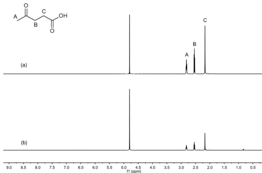
Figure 6. Typical 1 H NMR spectra. (a) LA standard and (b) LA product.
