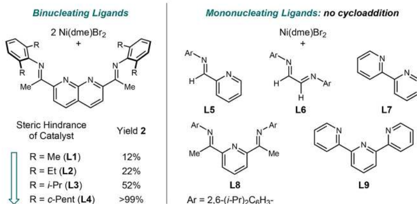
Fig. 1. Reaction development.
