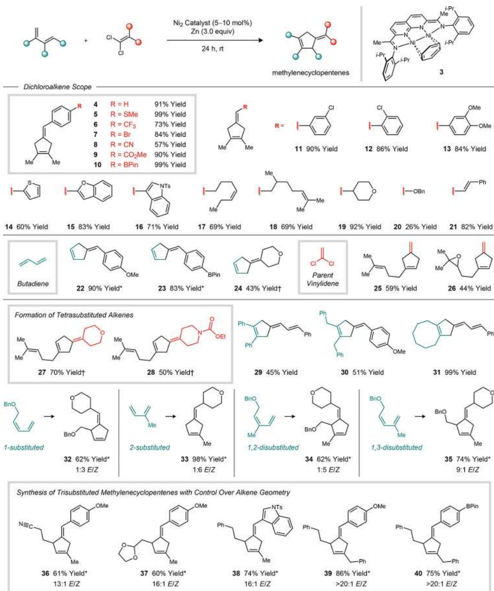
Fig. 2. Reaction scope.
