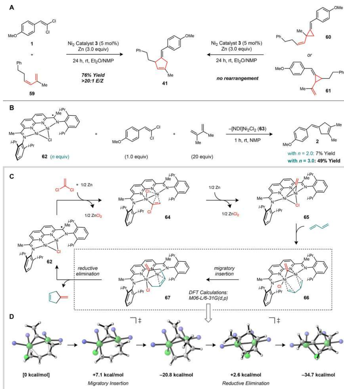
Fig. 4. Mechanistic investigations.
