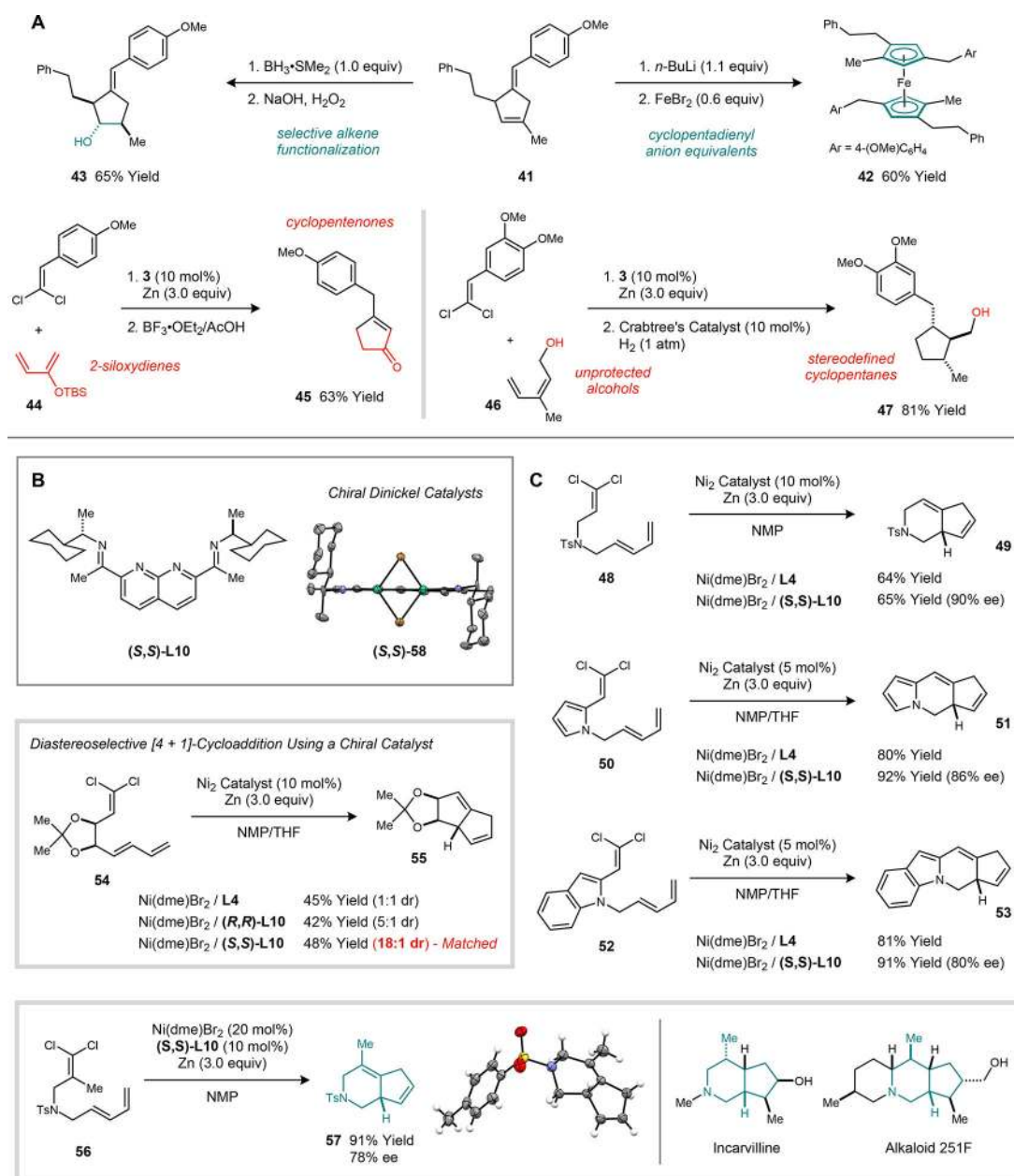
Fig. 3. Synthetic applications of the catalytic [4 + 1]-cycloaddition reaction.
