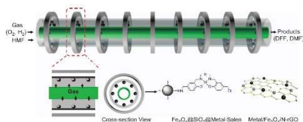
Figure 9. Tube-in-tube microreactor configuration for the solid catalyzed aerobic oxidation of HMF to DFF or hydrogenation of HMF to DMF. A gas permeable PTFE capillary ( d_c = 0.61 mm) was inserted in a wall-coated PTFE capillary ( d_c = 1 mm). The gas phase ( O_2 or H_2 ) was fed through the inner capillary and liquid through the outer capillary in co-current flow. Reproduced with permission of ref. [144] Copyright 2015 Springer Nature Publishing AG.
