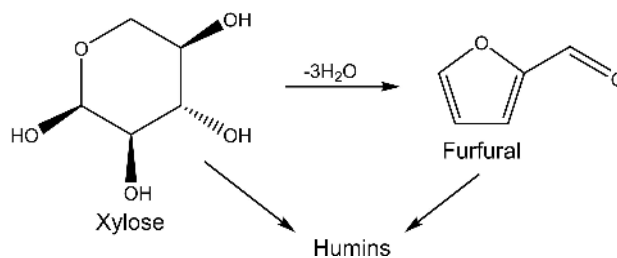
Scheme 2. Dehydration of xylose to furfural with the formation of humins as a typical byproduct.
