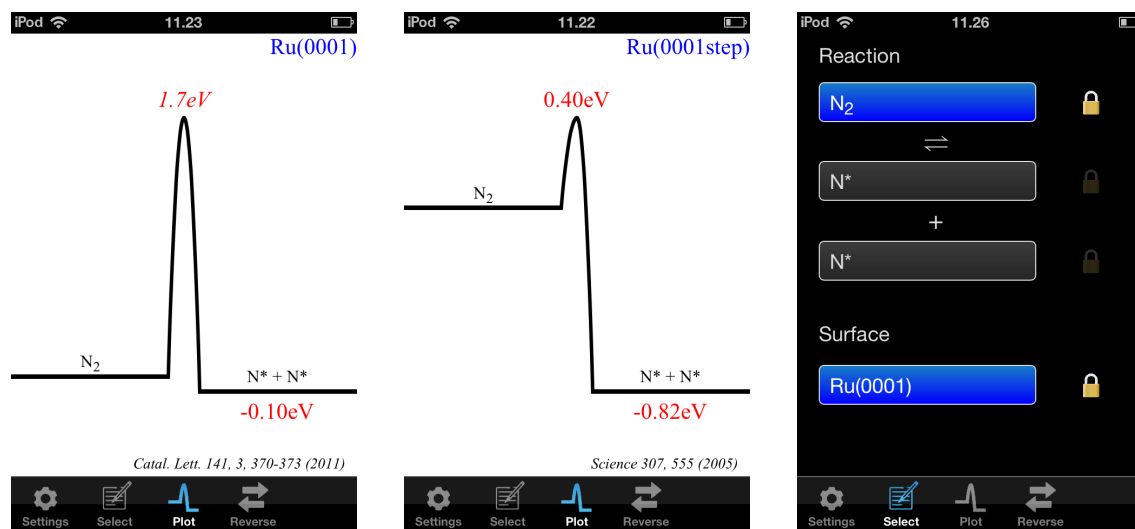
Figure 1. Screenshots from the app. Two leftmost panels: N_2 splitting on Ru(0001) and on stepped Ru(0001) , respectively. Right panel: In the select view the user can from dropdown menus choose the reaction parameters ( AB , A , B ) and the surface parameter. When a parameter has been selected the CatApp dynamically hides values of the unselected parameters for which neither DFT nor scaling energies are available.
