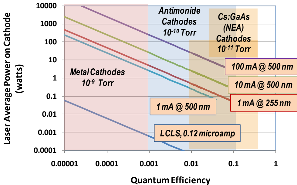
Figure 1: Plot of the average laser power vs. quantum efficiency to produce various average beam currents. The QE ranges for the general cathode types are shown along with their vacuum requirements.
