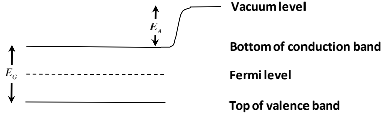
Figure 2: The energy levels of a simple semiconductor [33].
