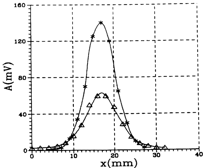
Fig. 6. The distribution of cathode signals of X-ray source position along the 10 mm diameter straw. (*) — single straw; ( \Delta ) — 44 straws. (a), (b) — cathode resistivity 30 and 70 kOhm/sq, respectively
