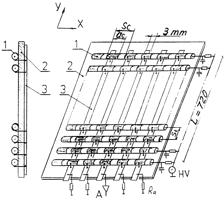
Fig.1. The layout of the prototype. 1 — straw with a_c wide ring strips; 2 — fiberglass support; 3 — strip bus for X-coordinate readout
