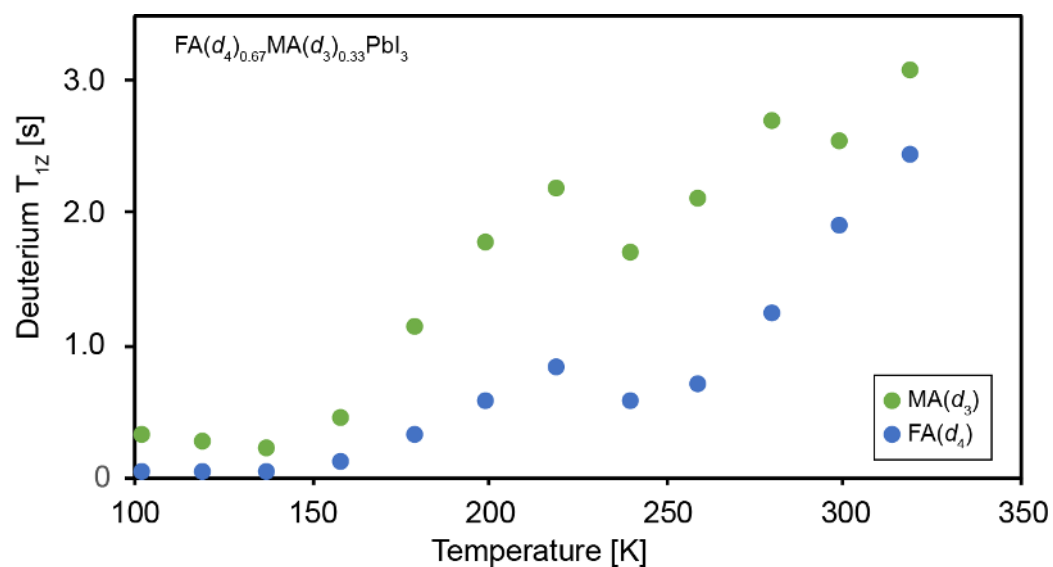
Figure S2. ^2\text{H} T_{12} relaxation in in \text{FA}(d_4)_{0.67}\text{MA}(d_3)_{0.33}\text{PbI}_3 as a function of temperature.
