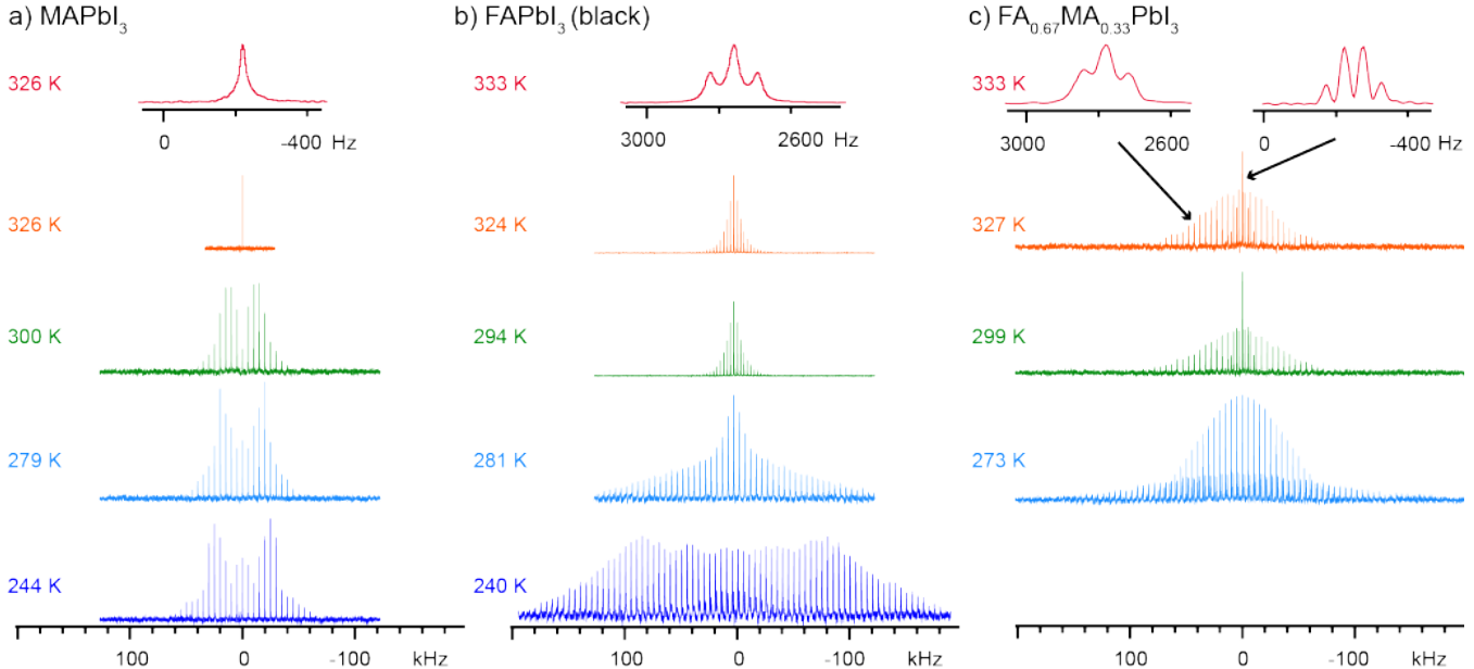
Figure 4. Solid-state ^{14}\text{N} echo-detected variable-temperature MAS NMR spectra. The MAS rate was either 3 or 5 kHz (between 240 and 327 K) and 20 kHz for the two top 333 K spectra in b) and c). The top insets (red) show a close-up of the central peak with a characteristic splitting due to the familiar J -coupling between the nitrogen and the proton.
