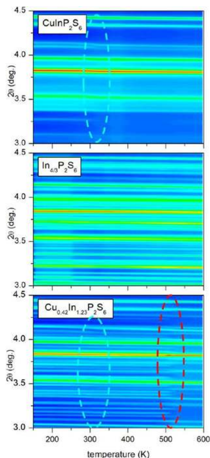
Figure 2. Contour plots of synchrotron X-ray diffraction (XRD) patterns ( \lambda = 0.117418 \text{ \AA} ) over the range of 150\text{--}600 \text{ K} for pure-phase \text{CuInP}_2\text{S}_6 and \text{In}_{4/3}\text{P}_2\text{S}_6 as well as mixed-phase \text{Cu}_{0.42}\text{In}_{1.23}\text{P}_2\text{S}_6 . The low-temperature transitions are circumscribed by a blue-colored dashed line, while the high-temperature transition is outlined in red.
