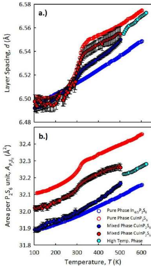
Figure 5. Comparison of the layer spacing and the in-plane area, normalized per P 2 S 6 unit, of pure In 4/3 P 2 S 6 and CuInP 2 S 6 (open blue and red symbols, respectively) and In 4/3 P 2 S 6 and CuInP 2 S 6 in a heterostructured alloy of average composition Cu 0.42 In 1.23 P 2 S 6 (solid blue and red symbols, respectively). Data for the high temperature phase are also shown (aqua symbols).
