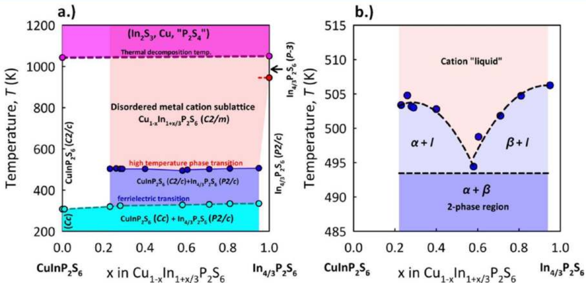
Figure 10. (a) Proposed phase diagram of the CuInP 2 S 6 /In 4/3 P 2 S 6 system based on thermodynamic characterization and high-resolution synchrotron data paired with the existing thermodynamic data of Gebesh et al.; 38 (b) expanded view of the binary eutectic region of the phase diagram (with respect to the cation sublattice).
