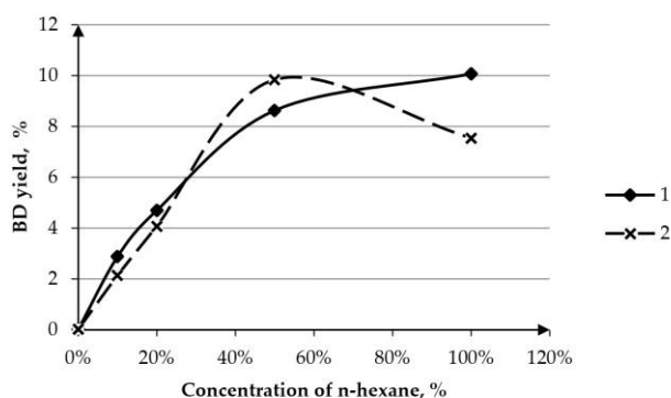
Fig. 6 Dependence of the BD yield on n-hexane concentration: [FA]:[IPA] = 1:5 mol.; T = 150 °C, τ = 180 min, 1 - TO, 2 - 37% aqueous solution of formaldehyde
