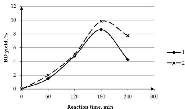
Fig. 5 Dependence of the BD yield on reaction time; [FA]:[IPA] = 1:5 mol.; T = 150 °C, [SO 3 H] = 0.6 eq/L, 1 - TO, 2 - 37 % aqueous solution of formaldehyde
