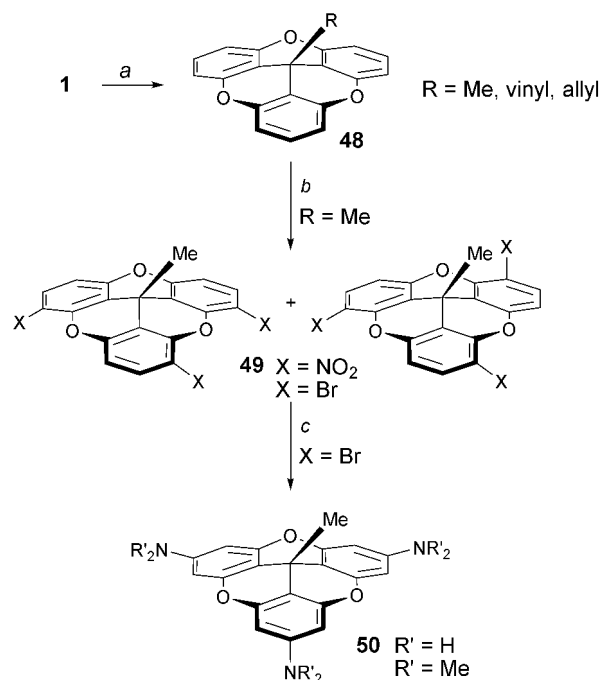
Scheme 16 Synthesis of trioxatricornan 50 . a: \text{MeLi-LiBr} , \text{Et}_2\text{O} , THF, 20^\circ\text{C} , 1 h or \text{CH}_2\text{CHMgBr} , THF, 20^\circ\text{C} , 7 h or \text{CH}_2\text{CHCH}_2\text{MgBr} , THF/ \text{Et}_2\text{O} , 0 to 20^\circ\text{C} , 16 h; b: \text{HNO}_3 or \text{Br}_2 , \text{CH}_3\text{COOH} , 80^\circ\text{C} , 30 min; c: \text{NaNH}_2 , liq \text{NH}_3 , THF, -78 to 20^\circ\text{C} , sealed tube, 19 h or \text{HNMe}_2 , n -BuLi, THF, -78 to 20^\circ\text{C} , sealed tube, 48 h.
