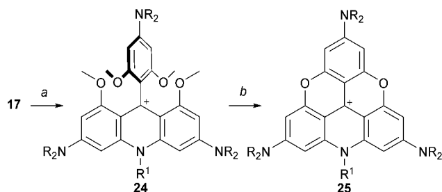
Scheme 8 Preparation of A_3\text{-ADOTA}^+ 25 . a: R^1\text{-NH}_2 , 20 °C, 4 days; b: Lil (10 equiv.), collidine, 180 °C, 2 h.
