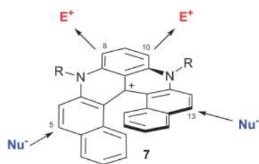
Fig. 4 Post-functionalization of cationic diaza[6]helicene 7 .
