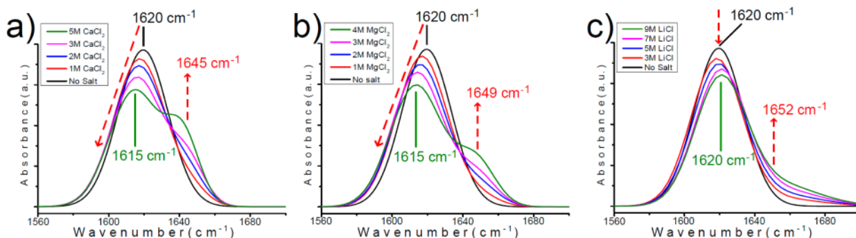
Figure 3. FTIR spectra of the amide I band for d -butyramide at (a) CaCl_2 concentrations from 0 to 5 M, (b) MgCl_2 from 0 to 4 M, and (c) LiCl from 0 to 9 M.
