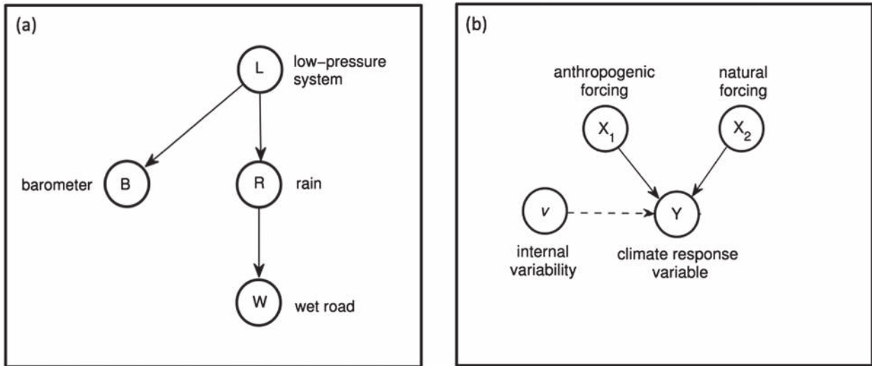
FIG. 1. Graphs representing dependencies (a) among the four variables (R, B, W, L) used in our illustrative example and (b) among forcings ( X_1 , X_2 ) and climate response Y. Dotted arrows represent dependency upon the unobserved variable v .
