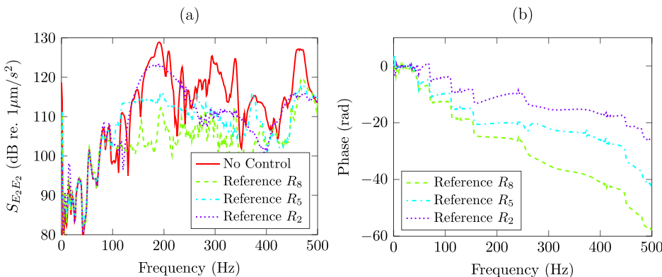
FIG. 5. (Color online) (a) Performance of the optimal causal feedforward controller and (b) phase response of the all-pass part of the optimal feedforward controller evaluated for three different reference sensors.
