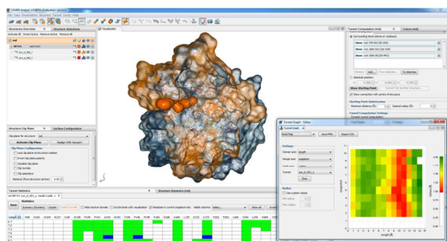
Fig. 1. The graphical user interface of the CAVER Analyst 1.0.
