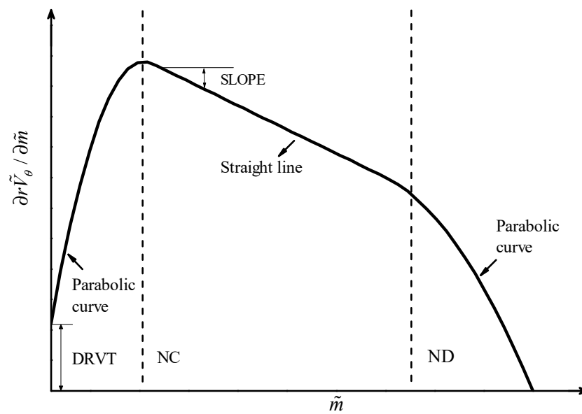
Figure 10. Blade loading distributions.
