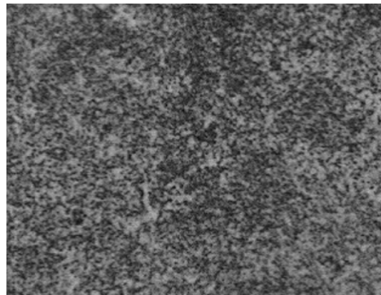
Fig. 3. P110 steel microstructure, magn. 1000x
