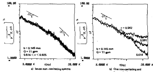
Fig. 16 Non-cavitating and cavitating energy spectra for prototype valve at a fixed opening and Q = 11 \text{ gpm}
