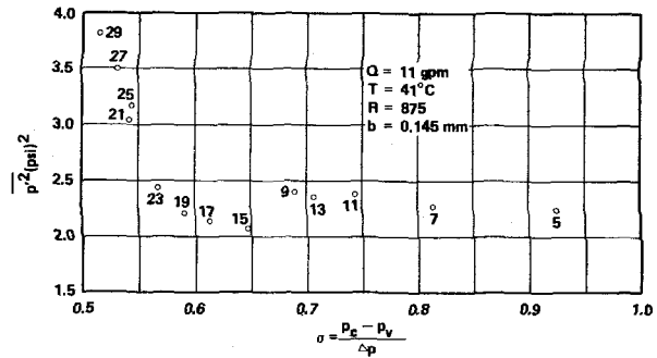
Fig. 15 Mean-square energy versus cavitation index for prototype valve at a fixed opening and Q = 11 \text{ gpm}
