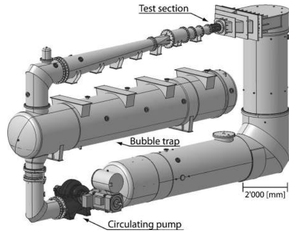
Fig. 1 EPFL high speed cavitation tunnel
