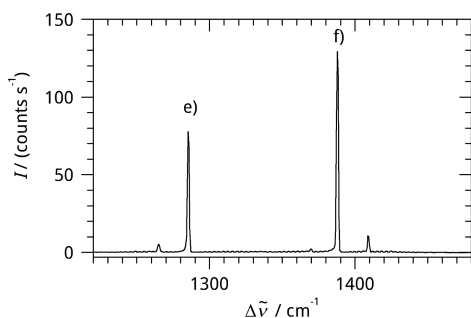
Figure 5. CERS spectrum of 1 bar \text{CO}_2 . Features (e) and (f) are labeled as in Figure 2; they represent the Q-branches of the \nu_1/2\nu_2^0 Fermi resonance pair.
