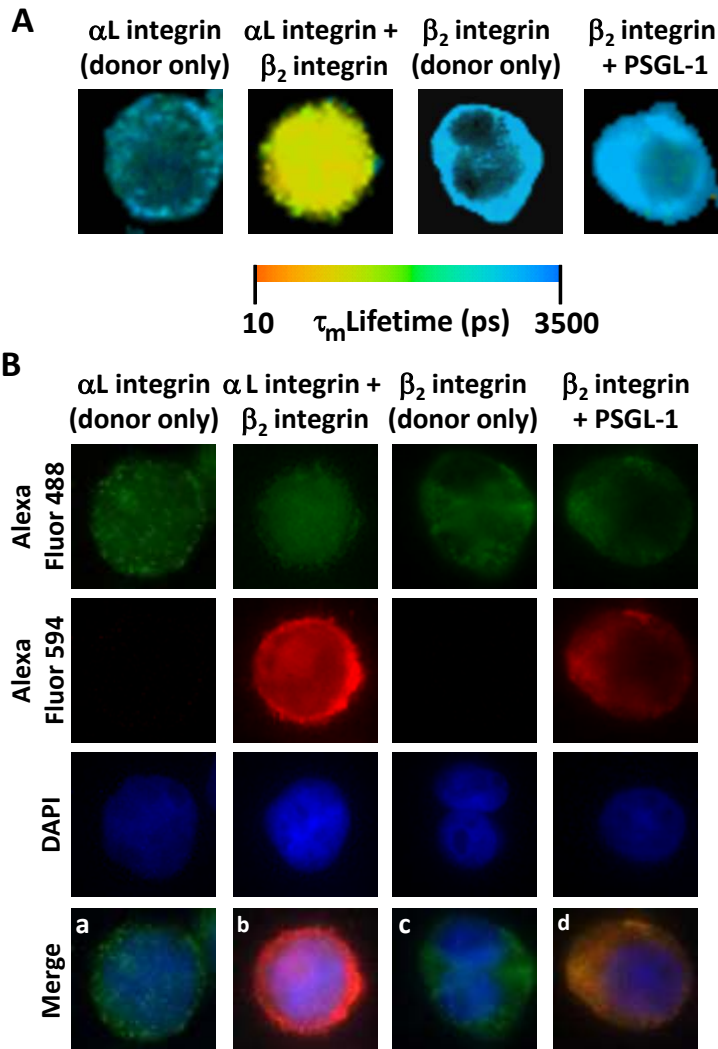
Supplemental Figure S2. \beta 2 integrin interacts with \alpha L integrin but not with PSGL-1 on the cellular membrane of Jurkat T cells. (A) Representation of interacting fraction \tau_m by pseudocolor images of the FLIM-FRET analysis of the interaction between \alpha L and \beta 2 integrins and \beta 2 integrin and PSGL-1. The color scale for the \tau_m lifetimes ranges from 10 to 3500 picoseconds (ps). As positive control \alpha L integrin was identified with the donor fluorophore (Alexa Fluor 488) and \beta 2 integrin with the acceptor fluorophore (Alexa Fluor 594). As a non-interacting control, \beta 2 integrin, was used as a donor and PSGL-1 as an acceptor. (B) Localization of \beta 2 integrin, \alpha L integrin and PSGL-1. Fixed cells were costained with (a) anti- \alpha L integrin antibody alone (clone TS1/22) (b) anti- \alpha L integrin antibody and anti- \beta 2 integrin polyclonal antibody (Quinn et al. , 2001) followed by an anti-mouse Alexa Fluor 488-conjugated and anti-rabbit Alexa Fluor 594-conjugated secondary antibodies, respectively. (c) anti- \beta 2 integrin antibody alone and (d) anti- \beta 2 integrin antibody and anti-PSGL-1(clone 13A9) followed by an anti-rabbit Alexa Fluor 488-conjugated and anti-mouse Alexa Fluor 594-conjugated secondary antibodies, respectively. The nucleus was stained with DAPI.
