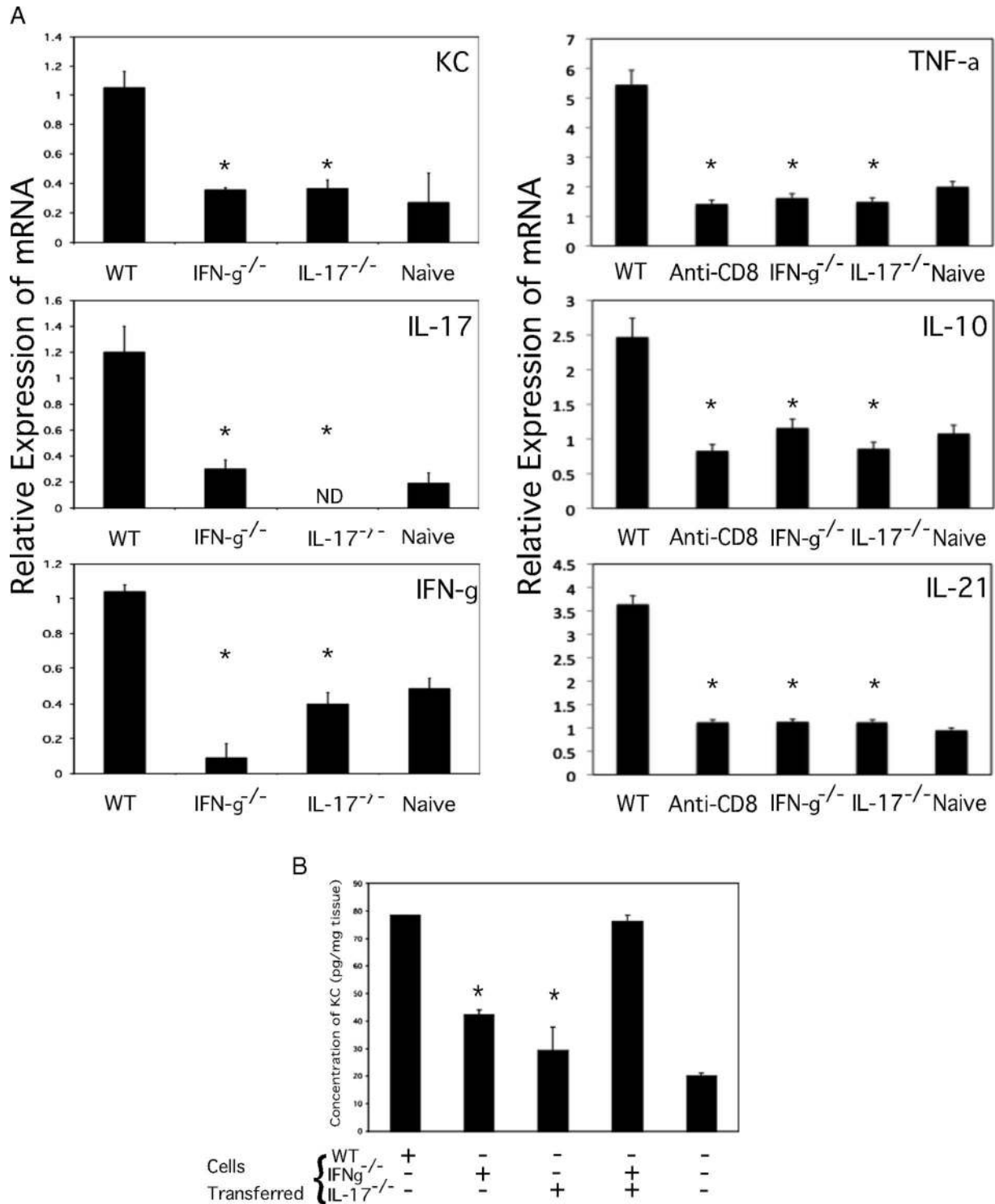
FIGURE 11. Both hapten-specific CD8 T cell-derived IFN- \gamma and IL-17 are required to stimulate proinflammatory cytokines in response to hapten challenge. A , Wild-type BALB/c, IFN- \gamma -/- , and IL-17 -/- mice were sensitized with 0.25% DNFB on days 0 and +1. On day +5, sensitized and nonsensitized naive mice were challenged with 0.2% DNFB, and challenged skin was excised for 6 h postchallenge. Whole cell RNA was prepared and used to assess mRNA expression of CXCL1, IL-17, IFN- \gamma , TNF- \alpha , IL-10, and IL-21 in the skin challenge site by quantitative RT-PCR. B , CD8 T cell donor BALB/c wild-type, IFN- \gamma -/- , and IL-17 -/- mice were depleted of CD4 T cells and sensitized with 0.25% DNFB on days 0 and +1. On day +4, groups of naive BALB/c mice ( n = 4 ) received 5 \times 10^6 LNC aliquots and were challenged with 0.2% DNFB. CXCL1 concentrations in the challenged skin 6 h later were determined by ELISA. The mean concentration \pm SEM is shown. Results are representative of two individual experiments. *, p < 0.02 . ND, Not detectable.
