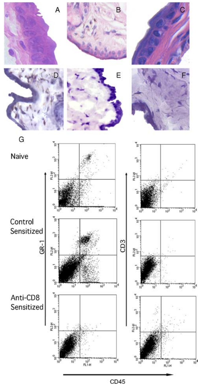
FIGURE 5. Presence of neutrophils but not CD8 T cells in the skin 6 h after hapten challenge of sensitized mice. BALB/c mice were treated with rat IgG or anti-CD8 mAb and then sensitized with 0.25% DNFB on days 0 and +1. On day +5, sensitized and nonsensitized naive mice were challenged with 0.2% DNFB. A–C, Challenged skin was excised 6 h postchallenge and formalin-fixed sections were stained with H&E. Representative images of sections from naive (A) and sensitized mice treated with control IgG (B) or CD8-depleting mAb (C) during sensitization are shown. Frozen sections were stained with Abs to detect neutrophils (D) and CD8 + cells (E) from mice treated with control IgG during sensitization and neutrophils (F) from mice depleted of CD8 T cells before sensitization. Magnification is at \times 400 . G, The challenged skin was excised and digested 6 h later and prepared cell suspensions were stained with FITC-labeled anti-CD45 mAb and PE-labeled anti-GR-1 mAb or anti-CD3 mAb and analyzed by flow cytometry. Results are representative of three individual experiments.
