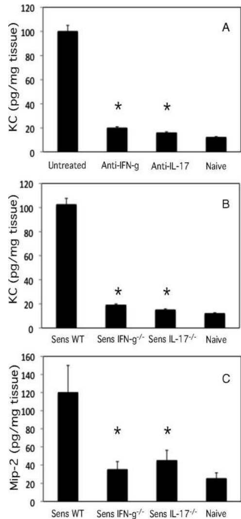
FIGURE 10. Induction of early CXCL1 and CXCL2 during elicitation of CHS requires IFN- \gamma and IL-17. A, On day +5, groups of DNFB-sensitized C57BL/6 mice were treated i.p. with 250 \mu g of rat IgG, anti-IFN- \gamma , or anti-IL-17 just before hapten challenge. B and C, Groups of wild-type BALB/c, IFN- \gamma^{-/-} , and IL-17 ^{-/-} mice ( n = 4 ) were sensitized with 0.25% DNFB on days 0 and +1. Challenged skin was excised at 6 h postchallenge, and prepared tissue homogenates were tested for levels of CXCL1 (A and B) and CXCL2 (C) by ELISA. The mean chemokine concentration \pm SEM for n = 4 individual mice is shown. Results are representative of two individual experiments. *, p < 0.03 .
