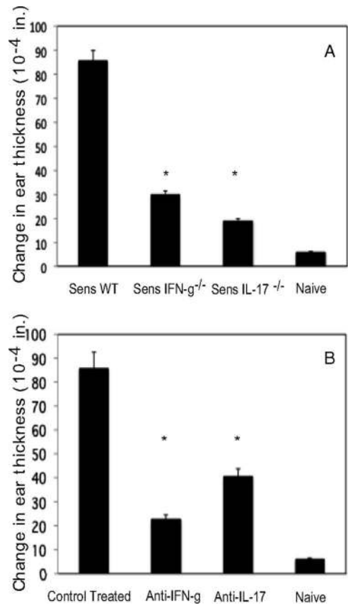
FIGURE 7. Both IFN- \gamma and IL-17 are required for elicitation of CHS. A, Groups of wild-type BALB/c, IFN- \gamma^{-/-} , and IL-17 -/- mice were sensitized with 0.25% DNFB on days 0 and +1. On day +5, sensitized mice and a group of nonsensitized/naive mice were challenged on the ears with 0.2% DNFB, and the change in ear thickness was measured 24 h later. B, Groups of sensitized C57BL/6 mice were treated with 350 \mu g of rat IgG, anti-IFN- \gamma , or anti-IL-17 i.v. just before hapten challenge. The mean increase in ear thickness following hapten challenge is shown in 10^{-4} in \pm SEM for groups of n = 4 mice. *, p < 0.001 .
