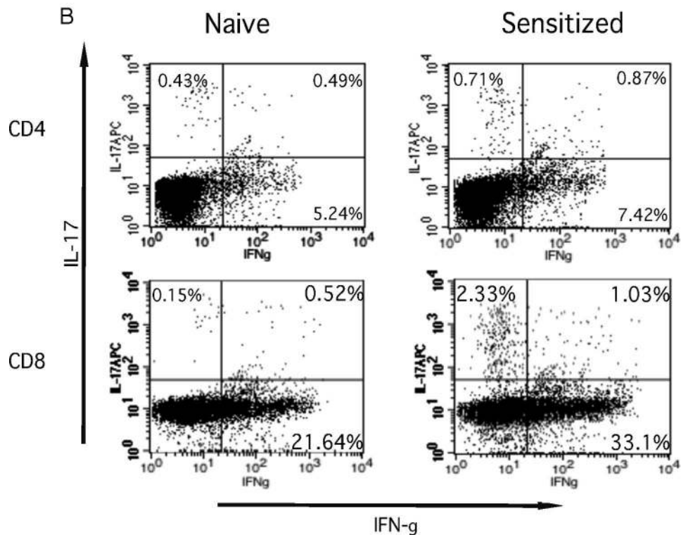
FIGURE 8. Hapten sensitization induces separate populations of CD8 T cells producing IFN- \gamma and IL-17. A , BALB/c wild-type, IFN- \gamma -/- , and IL-17 -/- mice were sensitized with 0.25% DNFB on days 0 and +1. On day +5, CD8 + T cells were prepared from skin draining lymph nodes and tested in ELISPOT assays with DNBS and unlabeled spleen cells to enumerate hapten-specific CD8 + T cells producing IFN- \gamma and IL-17. B , LNCs from naive or DNFB-sensitized mice were prepared on day +5 and stimulated with PMA and ionomycin and stained to detect intracellular IFN- \gamma and IL-17 by CD4 + and CD8 + T cell populations. Results are representative of four individual experiments in A and of two individual experiments in B . *, p < 0.01 .
