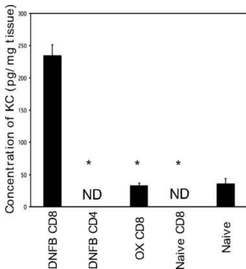
FIGURE 4. Hapten-primed CD8 T cells transfer Ag-challenge induction of early CXCL1/KC production to naive mice. T cell donor BALB/c mice were depleted of CD4 or CD8 T cells and sensitized with either 0.25% DNFB or 1% oxazolone on days 0 and +1. On day +4, groups of naive BALB/c mice ( n = 4 ) received 4 \times 10^6 LNC aliquots. Recipient mice were challenged with 0.2% DNFB and the concentration of CXCL1 in the challenged skin 6 h later was tested. The mean concentration \pm SEM for n = 4 individual mice is shown. Results are representative of two individual experiments. *, p < 0.05 . ND, Not detected.
