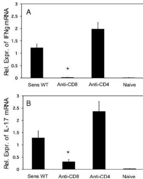
FIGURE 9. CD8 T cell mediated IFN- \gamma and IL-17 mRNA is expressed by 6 h in the Ag challenge site during elicitation of CHS. Groups of BALB/c mice ( n = 4 ) were treated with rat IgG, anti-CD4, or anti-CD8 mAb and then sensitized with 0.25% DNFB on days 0 and +1. On day +5, sensitized and nonsensitized naive mice were challenged with 0.2% DNFB and challenged skin was excised 6 h postchallenge. Whole cell RNA was prepared and used to assess mRNA expression of IFN- \gamma (A) and IL-17 (B) in the skin challenge site by quantitative RT/PCR. *, p < 0.05 .
