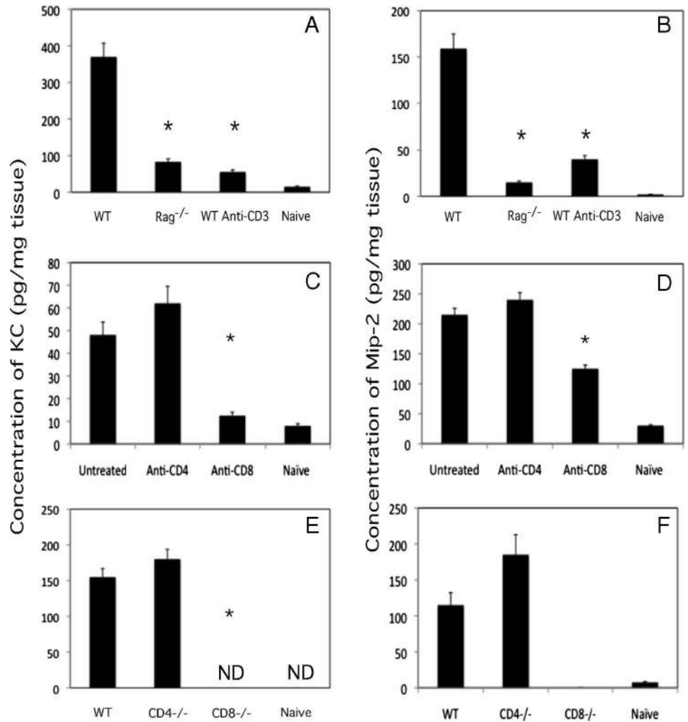
FIGURE 2. CD8 T cells mediate CXCL1/KC and CXCL2/MIP-2 production within 6 h of Ag challenge of sensitized mice. A and B , Groups of wild-type C57BL/6 were treated with rat IgG or anti-CD3 mAb to deplete T cells. These mice and a group of B6.RAG-1 -/- mice were sensitized and challenged with DNFB. C and D , Groups of BALB/c mice ( n = 4) were depleted of CD4 or CD8 T cells before DNFB sensitization and challenge. E and F , Groups of wild-type C57BL/6, B6.CD4 -/- , and B6.CD8 -/- mice were sensitized and challenged with DNFB. Tissue homogenates were prepared 6 h after DNFB challenge of sensitized and naive mice and tested by ELISA for production of CXCL1 ( A , C , and E ) or CXCL2 ( B , D , and F ). The mean concentration of chemokine ± SEM for n = 4 individual mice in each group is shown. *, p ≤ 0.01. ND, Not detected.
