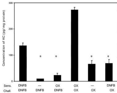
FIGURE 3. CXCL1/KC production 6 h after skin challenge of sensitized mice is Ag-specific. Groups of BALB/c mice were sensitized with either 0.25% DNFB or 1% oxazolone (OX) on days 0 and +1 and challenged with either 0.2% DNFB or 1% oxazolone as indicated. Challenged skin was removed 6 h postchallenge, and prepared tissue homogenates were tested for concentrations of CXCL1 by ELISA. *, p \leq 0.005 .
