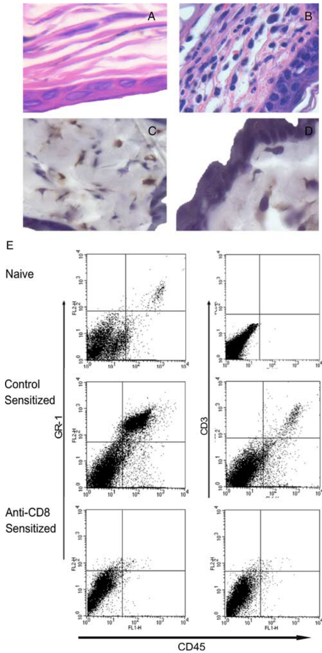
FIGURE 6. Both neutrophils and CD8 T cells infiltrate the skin 18 h after hapten challenge. DNFB-sensitized and nonsensitized BALB/c mice were challenged with 0.2% DNFB and challenged skin was excised 18 h later and fixed in formalin. Prepared sections were stained with H&E. Representative images of sections from naive (A) and sensitized (B) mice are shown. Skin from DNFB-sensitized and -challenged mice was also fixed in OCT and frozen, and prepared sections were stained with Abs to detect neutrophils (C) and CD8 + T cells (D). Magnification is at \times 400 . E, The skin was excised 18 h after challenge, digested, and prepared cell suspensions were stained with FITC-labeled anti-CD45 mAb and PE-labeled anti-GR-1 mAb or anti-CD3 mAb and analyzed by flow cytometry. Results are representative of three individual experiments.
