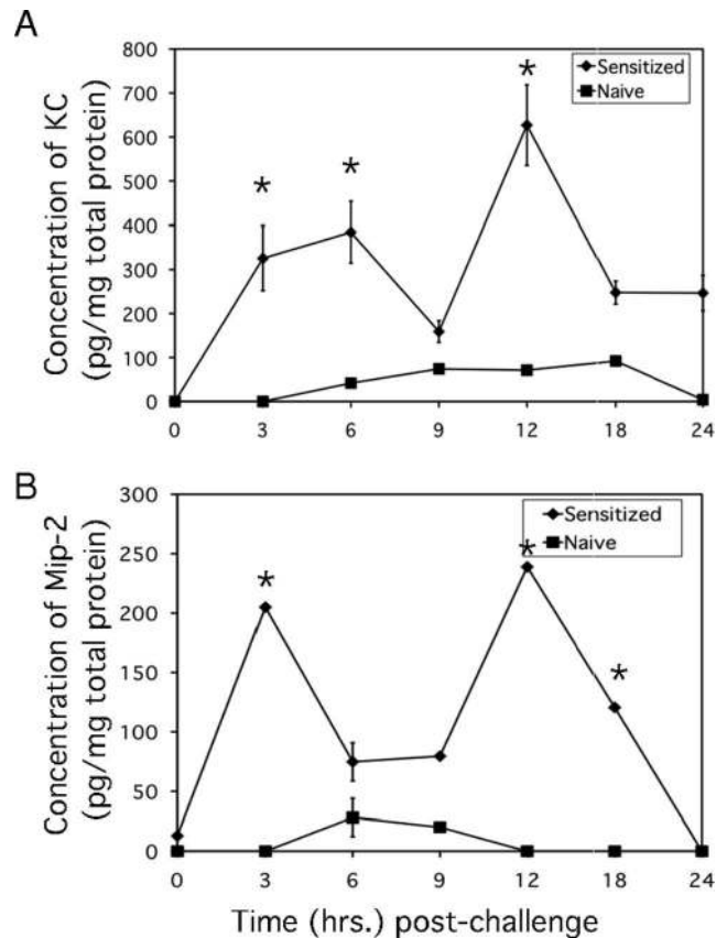
FIGURE 1. Rapid production of CXCL1/KC and CXCL2/MIP-2 in Ag-challenged skin of sensitized mice. BALB/c mice were sensitized with 0.25% DNFB on days 0 and +1. On day +5 after sensitization, mice were challenged on a shaved square area of trunk skin with 0.2% DNFB. Challenged areas of skin were removed from DNFB-sensitized ( \blacklozenge ) or nonsensitized ( \blacksquare ) mice at the indicated times postchallenge and prepared tissue homogenates were tested for concentrations of CXCL1 (A) or CXCL2 (B) by ELISA. The mean concentration \pm SEM for n = 4 individual mice per time point is shown. *, p \leq 0.01 .
