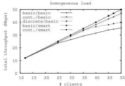
Fig. 1. Performance comparison under varying offered load, where 10 APs are deployed, and each client generates 1Mbps demand.
