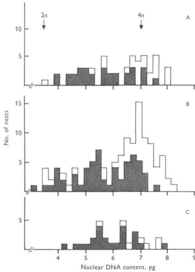
Fig. 2. Nuclear DNA content and [ ^3\text{H} ]thymidine incorporation in nests of 1, 2 and 4 interstitial cells. Five hydra were pulse-labelled with [ ^3\text{H} ]thymidine ( 10 \mu\text{Ci/ml} ) and macerated 30 min later. The maceration preparation was stained with the fluorescent Feulgen reagent bisaminophenyl-oxdiazole and the nuclear DNA content of individual cells determined by microfluorimetry. In a second step the same cells were assayed for [ ^3\text{H} ]thymidine incorporation by autoradiography. DNA values for different cells in the same nest were always very similar as was the level of [ ^3\text{H} ]thymidine incorporation. A, B, and C, 1, 2, and 4 cells/nest, respectively; 2n and 4n DNA values were determined on mitotic cells in metaphase and telophase; filled bars represent nuclei labelled with [ ^3\text{H} ]thymidine.
